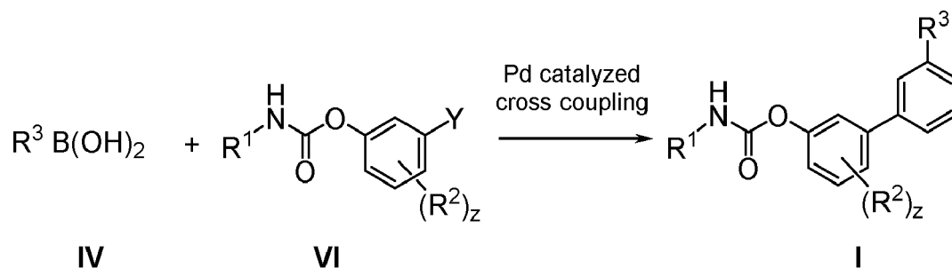
Scheme III: Synthesis of compounds of Formula I
