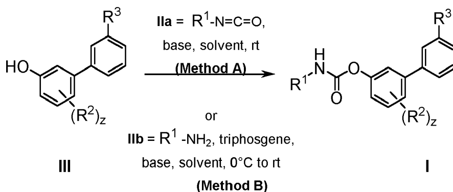
Scheme I: Synthesis of compounds of Formula I (Method A and B)
