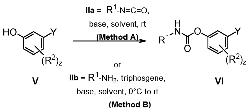
Scheme IV: Synthesis of compounds of Formula VI
