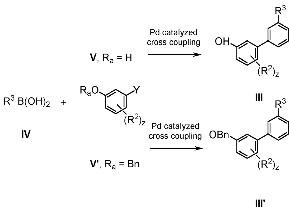
Scheme II: Synthesis of compounds of Formula III or the corresponding benzyl ethers III'
