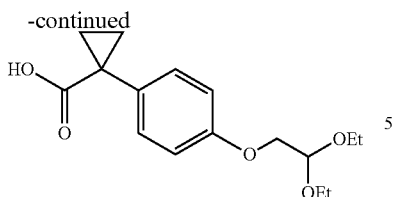
1-[4-(2,2-Diethoxy-ethoxy)-phenyl]-cyclopropanecarboxylic acid
