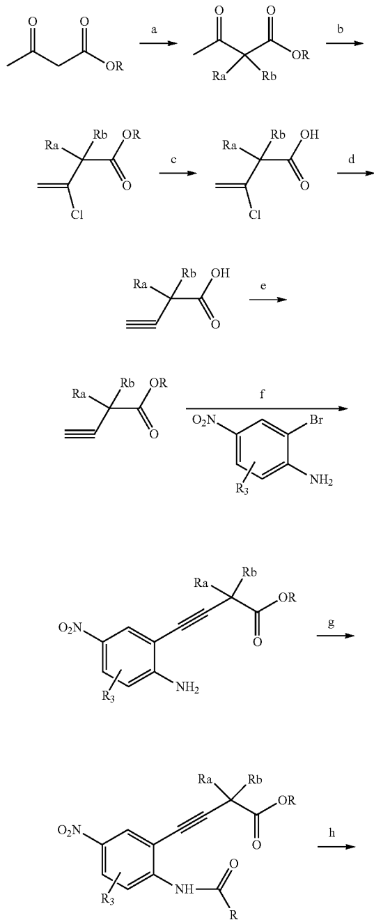
Scheme 31
