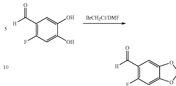
6-Fluoro-benzo[1,3]dioxole-5-carbaldehyde
