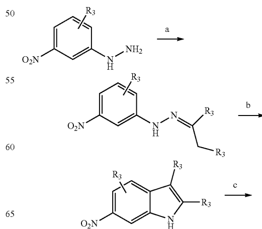
Scheme 12
