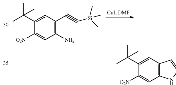
5-tert-Butyl-6-nitro-1H-indole
