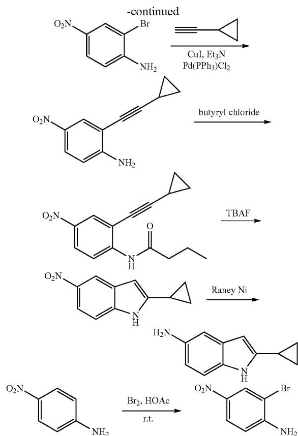
2-Bromo-4-nitroaniline
