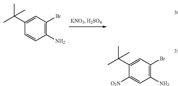
2-Bromo-4-tert-butyl-5-nitro-phenylamine
