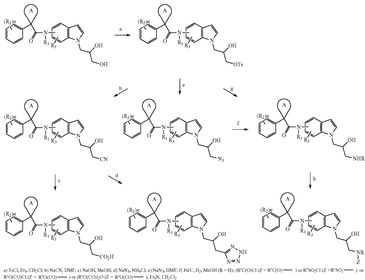
Scheme 40
