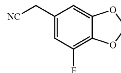
2-(7-Fluorobenzo[d][1,3]dioxol-5-yl)acetonitrile
