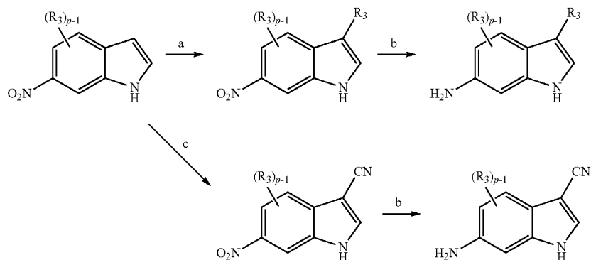
Scheme 15
