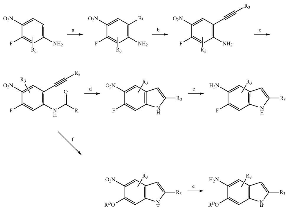
Scheme 18
