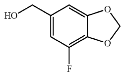
(7-Fluoro-benzo[1,3]dioxol-5-yl)-methanol
