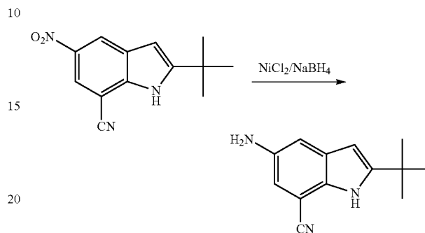
5-Amino-2-tert-butyl-1H-indole-7-carbonitrile
