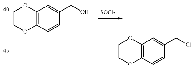
6-Chloromethyl-2,3-dihydro-benzo[1,4]dioxine
