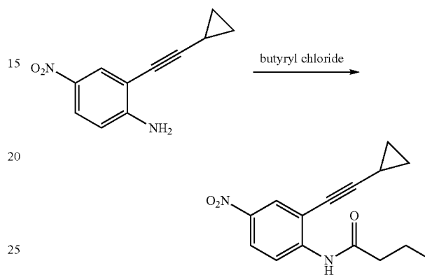
N-(2-(Cyclopropylethynyl)phenyl)-4-nitrobutyramide
