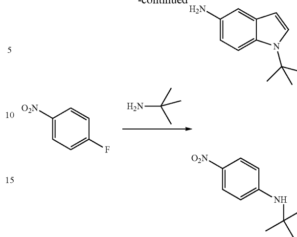
N-tert-Butyl-4-nitroaniline
