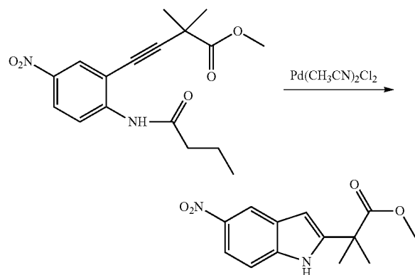
Methyl 2-methyl-2-(5-nitro-1H-indol-2-yl)propanoate
