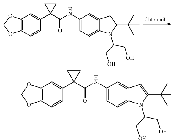
1-(Benzo[d][1,3]dioxol-5-yl)-N-(2-tert-butyl-1-(1,3-dihydroxypropan-2-yl)-1H-indol-5-yl)cyclopropanecarboxamide
