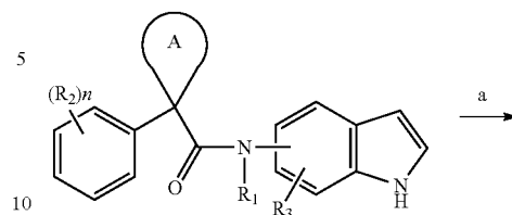
Scheme 37
