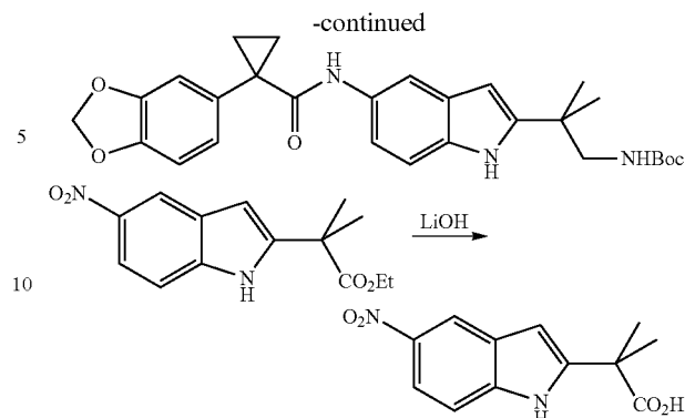
2-Methyl-2-(5-nitro-1H-indol-2-yl)propanoic acid
