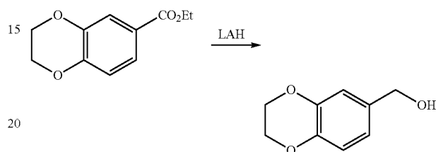
(2,3-Dihydro-benzo[1,4]dioxin-6-yl)-methanol
