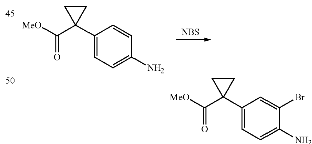
Methyl 1-(4-amino-3-bromophenyl)cyclopropanecarboxylate
