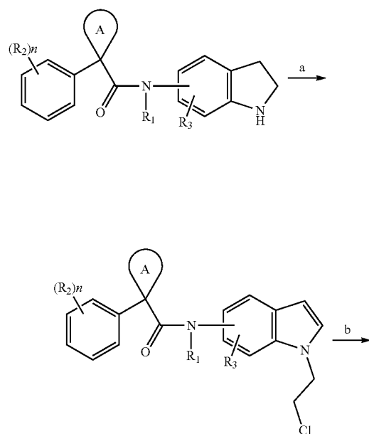
Scheme 41
