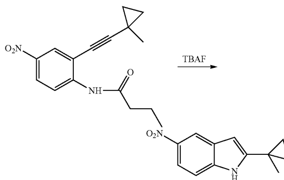
2-(1-Methylcyclopropyl)-5-nitro-1H-indole
