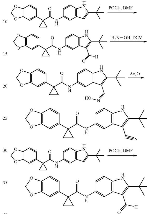
1-(Benzo[d][1,3]dioxol-5-yl)-N-(2-tert-butyl-3-formyl-1H-indol-5-yl)cyclopropane-carboxamide
