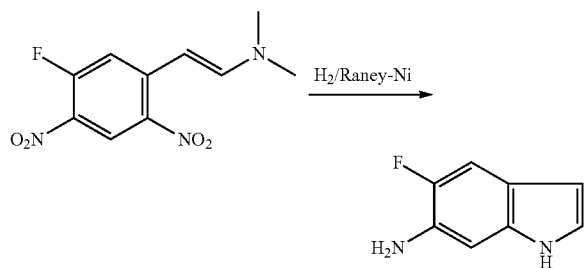
5-Fluoro-1H-indol-6-amine
