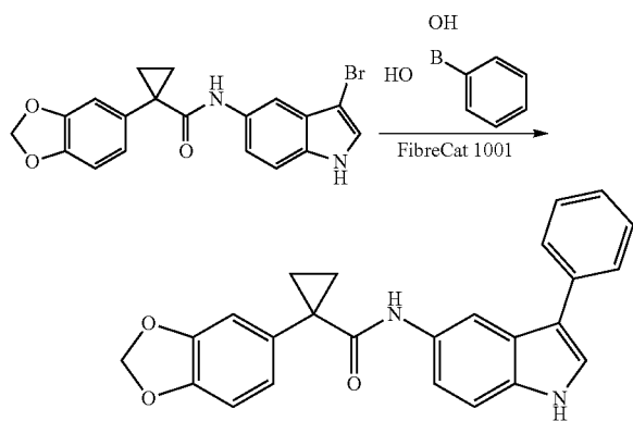
1-(Benzo[d][1,3]dioxol-5-yl)-N-(3-phenyl-1H-indol-5-yl)cyclopropanecarboxamide
