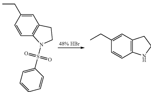
5-Ethylindoline
