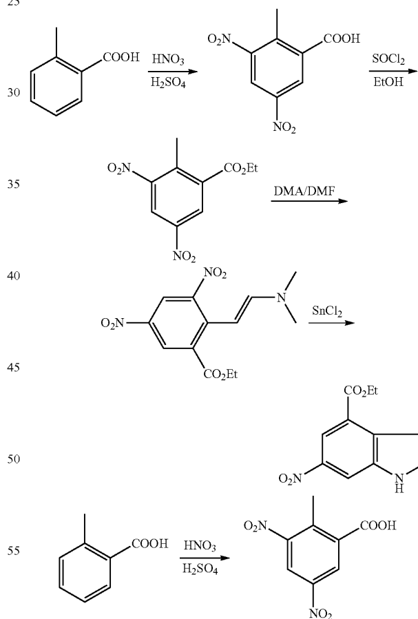
2-Methyl-3,5-dinitrobenzoic acid
