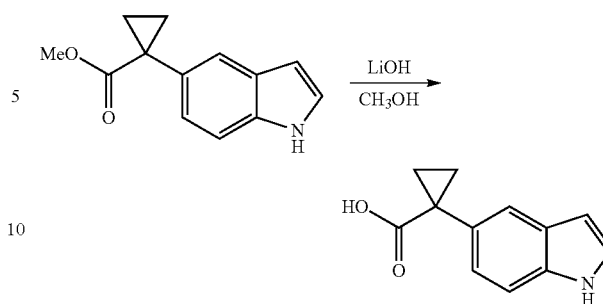
1-(1H-Indol-5-yl)cyclopropanecarboxylic acid
