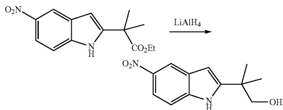
2-Methyl-2-(5-nitro-1H-indol-2-yl)propan-1-ol
