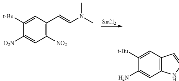
5-tert-Butyl-1H-indol-6-amine
