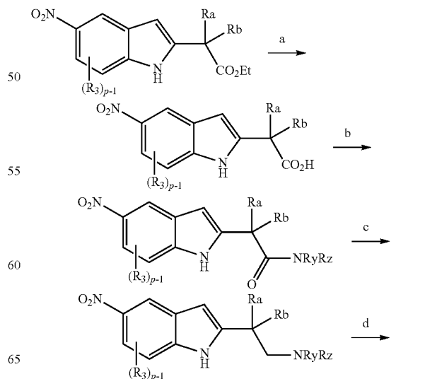
Scheme 26
