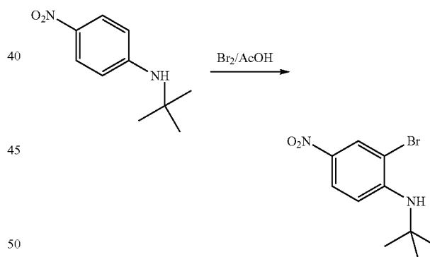
(2-Bromo-4-nitro-phenyl)-tert-butyl-amine
