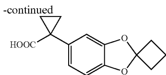
1-(Spiro[benzo[d][1,3]dioxole-2,1'-cyclobutane]-5-yl)cyclopropane carboxylic acid
