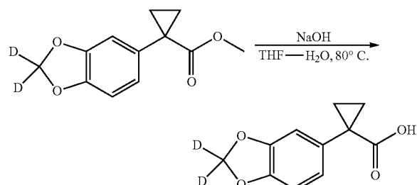
1-(2,2-Dideuteriumbenzo[d][1,3]dioxol-5-yl)cyclopropanecarboxylic acid
