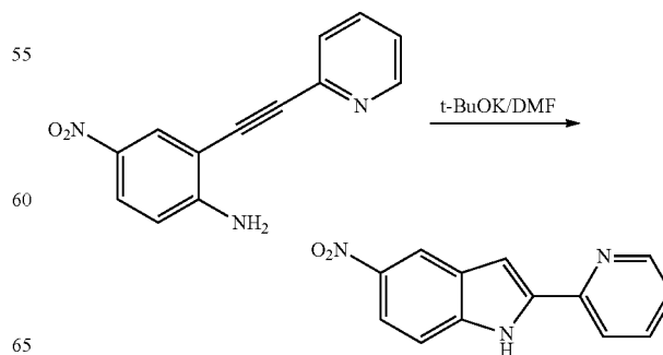
Example 46: 2-(Pyridin-2-yl)-1H-indol-5-amine
