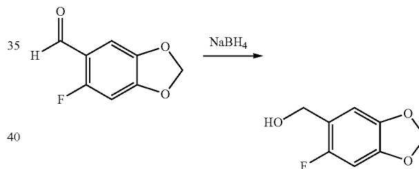
(6-Fluoro-benzo[1,3]dioxol-5-yl)-methanol
