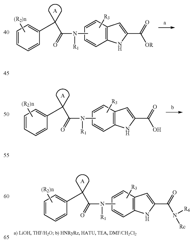
Scheme 32
