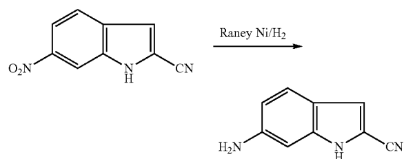
6-Amino-1H-indole-2-carbonitrile
