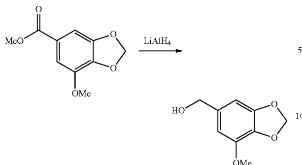
(7-Methoxybenzo[d][1,3]dioxol-5-yl)methanol
