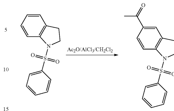
1-(1-(Phenylsulfonyl)indolin-5-yl)ethanone
