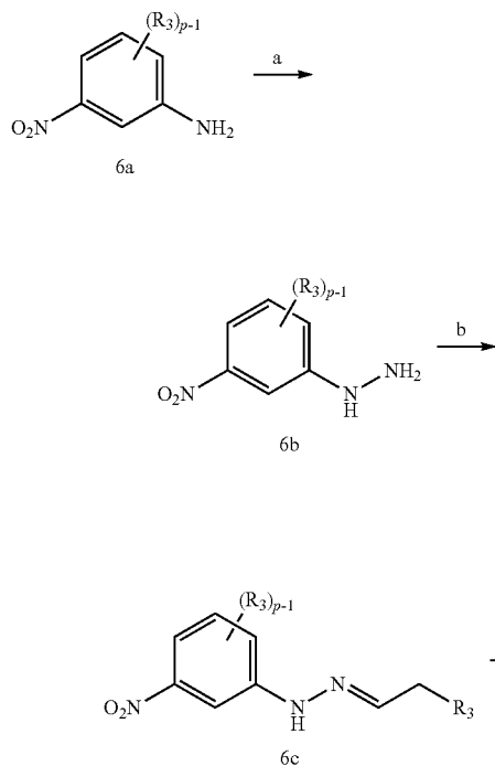
Scheme 6
