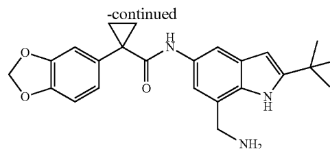
N-(7-(Aminomethyl)-2-tert-butyl-1H-indol-5-yl)-1-(benzo[d][1,3]dioxol-5-yl)cyclopropanecarboxamide
