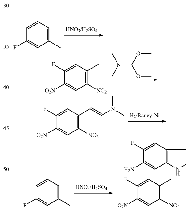
Example 56: 5-Fluoro-1H-indol-6-amine
