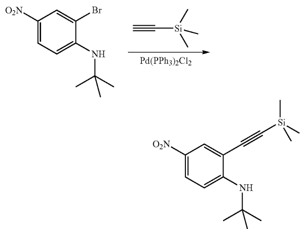
tert-Butyl-(4-nitro-2-trimethylsilanylethynyl-phenyl)-amine
