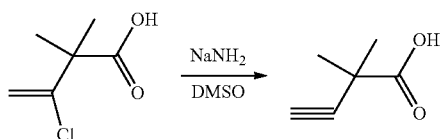
2,2-Dimethylbut-3-ynoic acid
