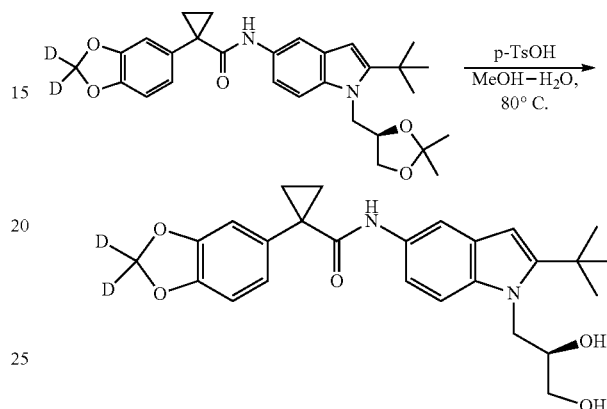
(R)—N-(2-tert-Butyl-1-((2,3-dihydroxypropyl)-1H-indol-5-yl)-1-(2,2-dideuteriumbenzo[d][1,3]dioxol-5-yl)cyclopropanecarboxamide
