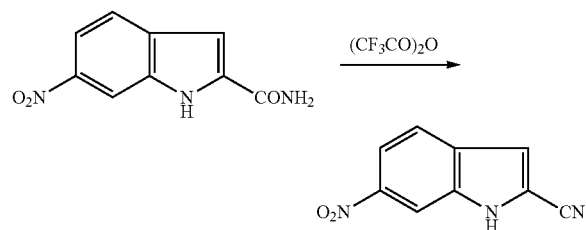
4-Nitro-1H-indole-2-carbonitrile and 6-nitro-1H-indole-2-carbonitrile
