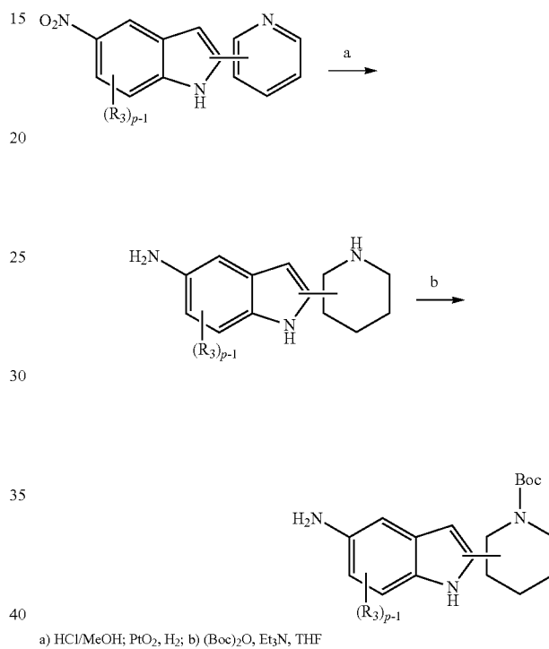
Scheme 29
