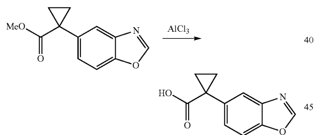
1-(Benzo[d]oxazol-5-yl)cyclopropanecarboxylic acid
