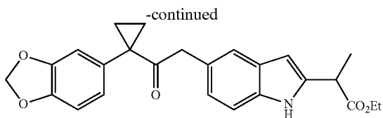
Ethyl 2-(5-(1-(benzo[d][1,3]dioxol-5-yl)cyclopropanecarboxamido)-1H-indol-2-yl)propanoate
