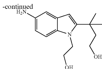
3-[5-Amino-1-(2-hydroxy-ethyl)-1H-indol-2-yl]-3-methyl-butan-1-ol
