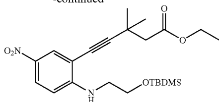
5-{2-[2-(tert-Butyl-dimethyl-silanyloxy)-ethyl-amino]-5-nitro-phenyl}-3,3-dimethyl-pent-4-ynoic acid ethyl ester
