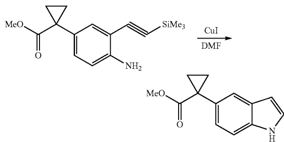
Methyl 1-(1H-indol-5-yl)cyclopropanecarboxylate
