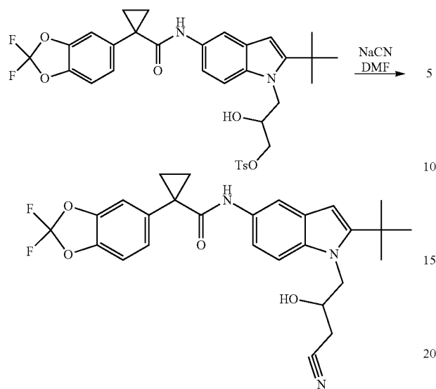
N-(2-tert-Butyl-1-(3-cyano-2-hydroxypropyl)-1H-indol-5-yl)-1-(2,2-difluorobenzo[d][1,3]dioxol-5-yl)cyclopropanecarboxamide
