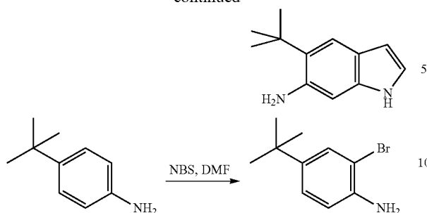
2-Bromo-4-tert-butyl-phenylamine
