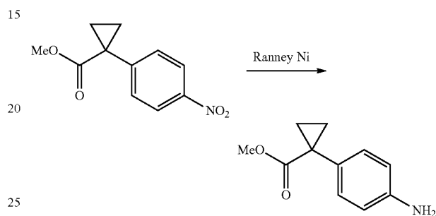
Methyl 1-(4-aminophenyl)cyclopropanecarboxylate
