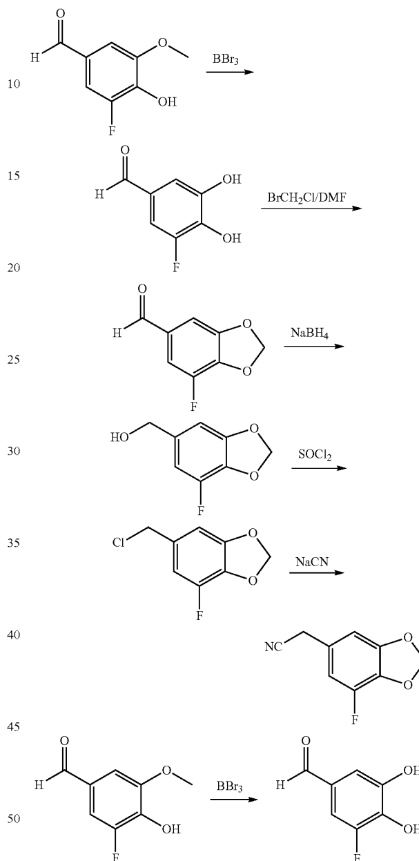
3-Fluoro-4,5-dihydroxy-benzaldehyde
