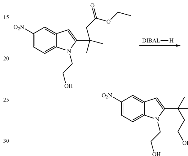
3-[1-(2-Hydroxy-ethyl)-5-nitro-1H-indol-2-yl]-3-methyl-butan-1-ol
