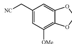
2-(7-Methoxybenzo[d][1,3]dioxol-5-yl)acetonitrile
