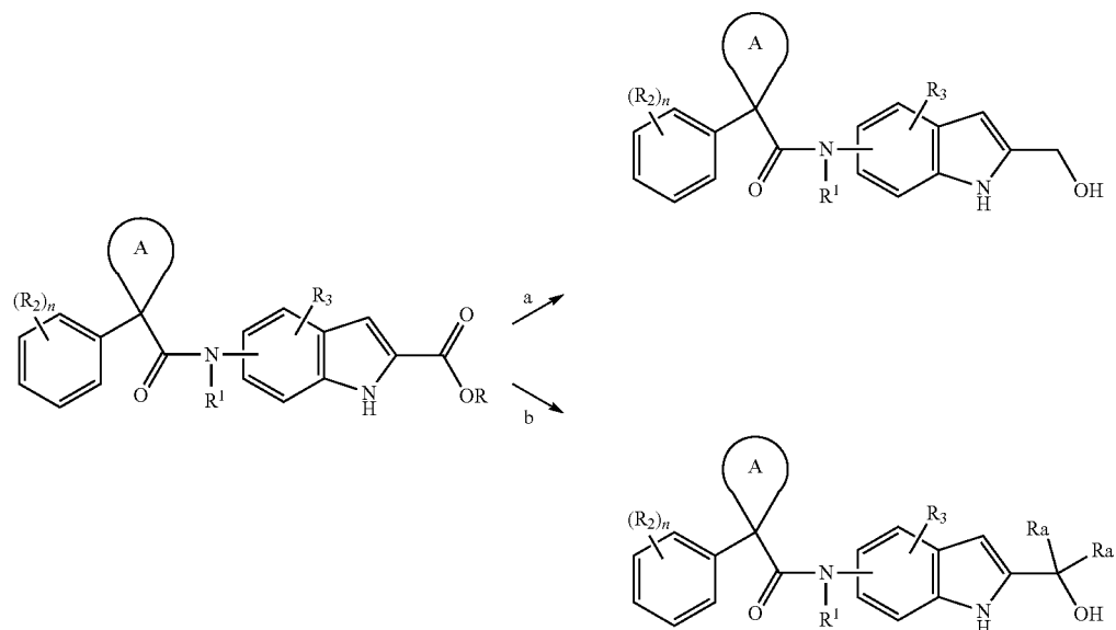
Scheme 33
