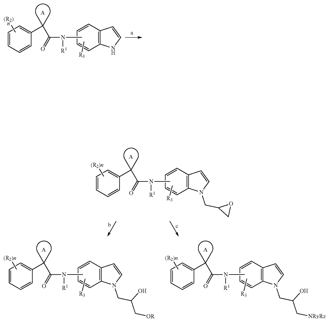
Scheme 39
