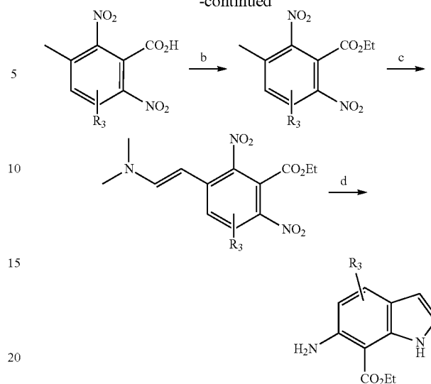
Scheme 11
