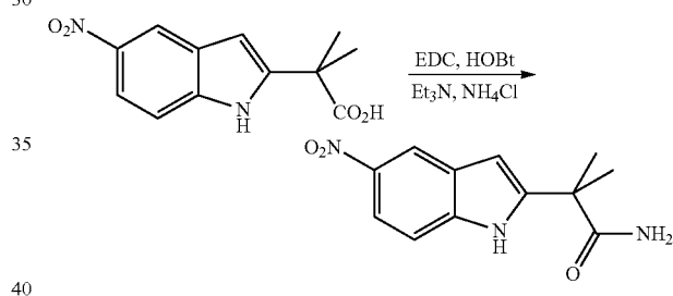
2-Methyl-2-(5-nitro-1H-indol-2-yl)propanamide
