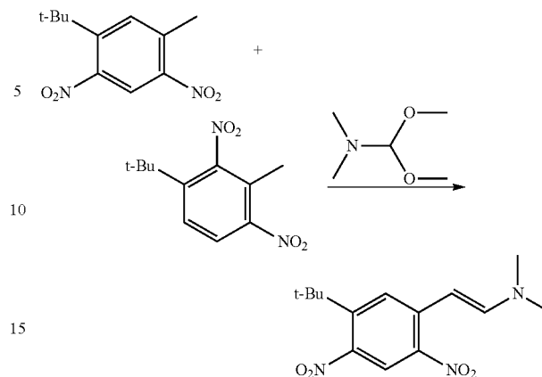
(E)-2-(5-tert-Butyl-2,4-dinitrophenyl)-N,N-dimethylethenamine
