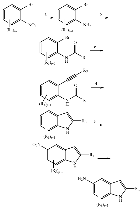
Scheme 23
