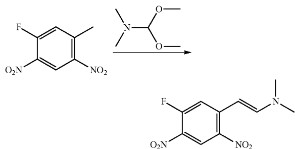
(E)-2-(5-Fluoro-2,4-dinitrophenyl)-N,N-dimethylethanamine
