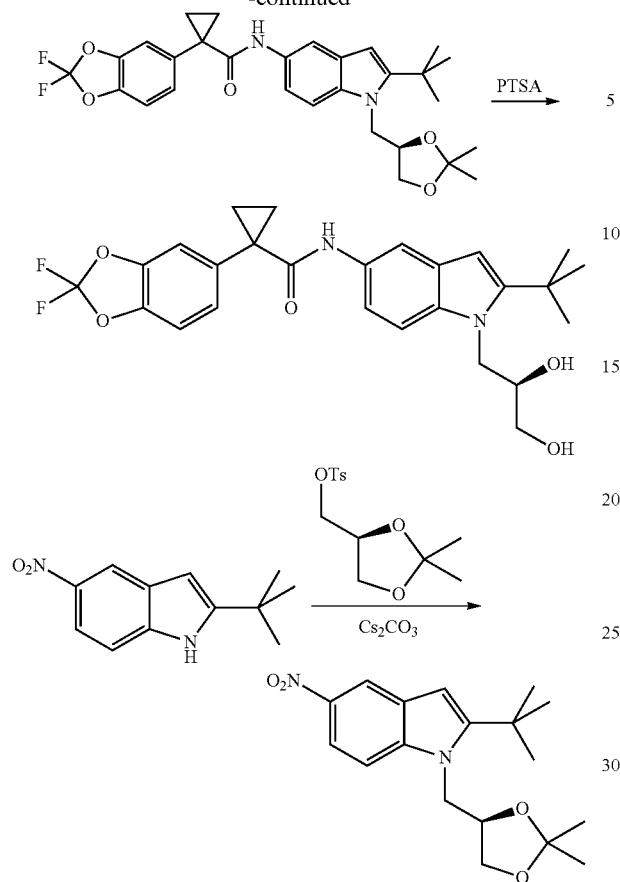
(R)-2-tert-Butyl-1-((2,2-dimethyl-1,3-dioxolan-4-yl)methyl)-5-nitro-1H-indole
