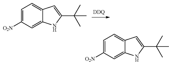
2-tert-Butyl-6-nitro-1H-indole
