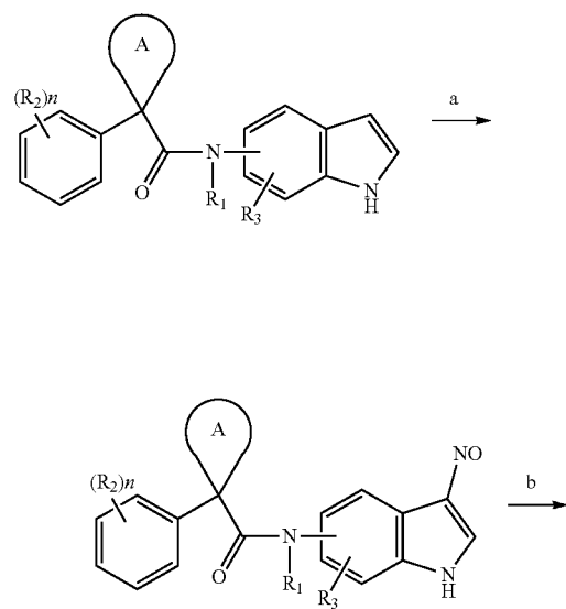
Scheme 34
