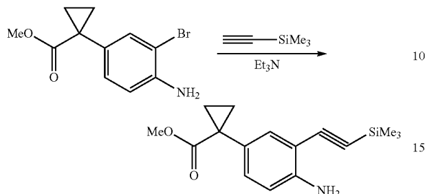
Methyl 1-(4-amino-3-((trimethylsilyl)ethynyl)phenyl)cyclopropanecarboxylate
