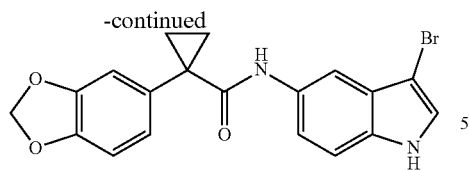
1-(Benzo[d][1,3]dioxol-5-yl)-N-(3-bromo-1H-indol-5-yl)cyclopropanecarboxamide
