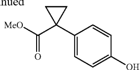
1-(4-Hydroxy-phenyl)-cyclopropanecarboxylic acid methyl ester
