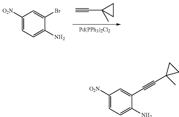
2-((1-Methylcyclopropyl)ethynyl)-4-nitroaniline
