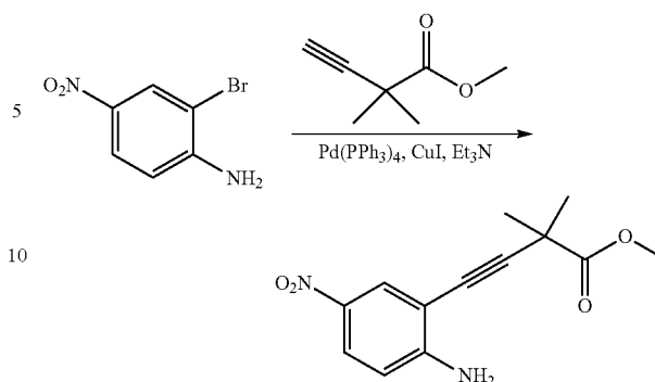
Methyl 4-(2-amino-5-nitrophenyl)-2,2-dimethylbut-3-ynoate
