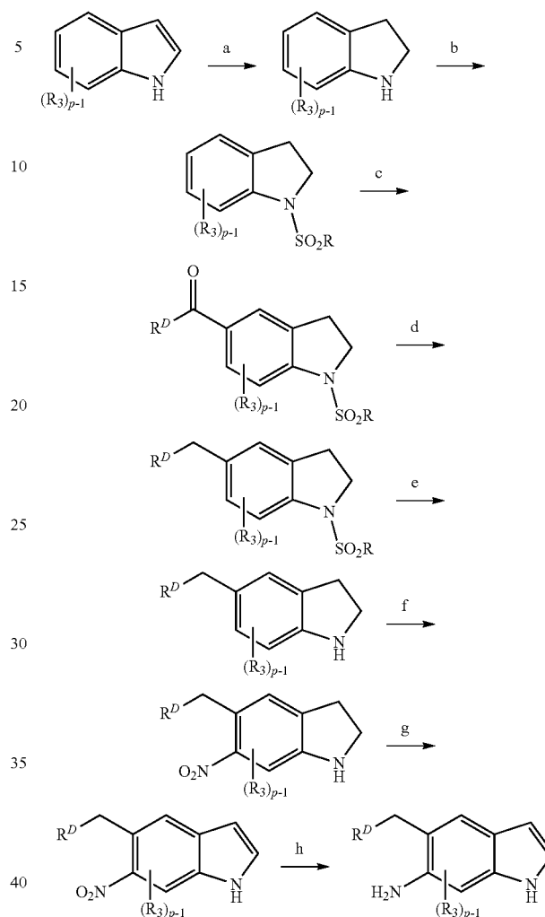
Scheme 14
