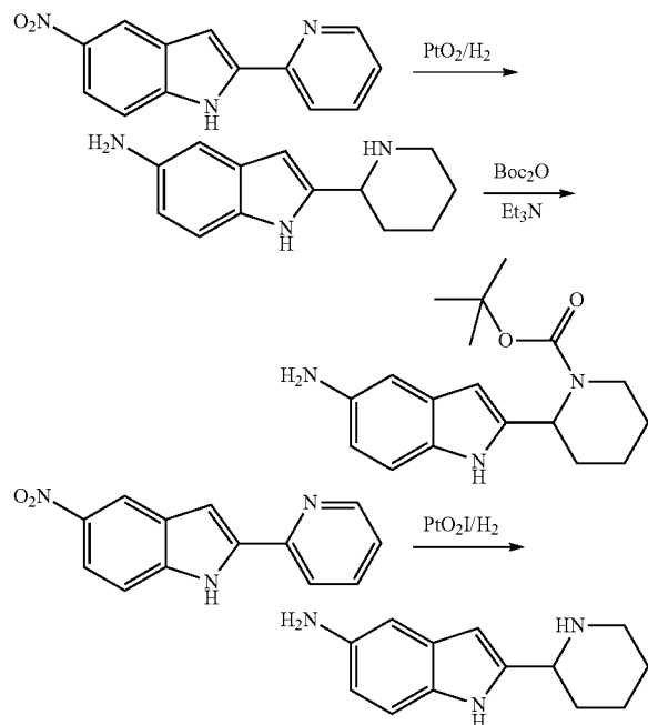
2-(Piperidin-2-yl)-1H-indol-5-amine
