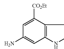
Ethyl 6-amino-1H-indole-4-carboxylate
