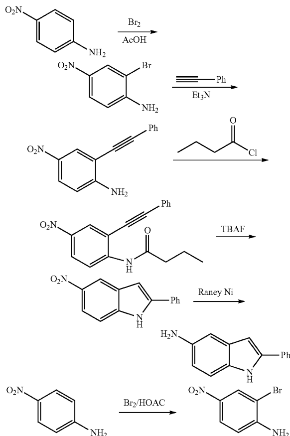
2-Bromo-4-nitroaniline
