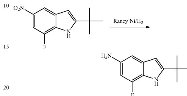
2-tert-Butyl-7-fluoro-1H-indol-5-amine
