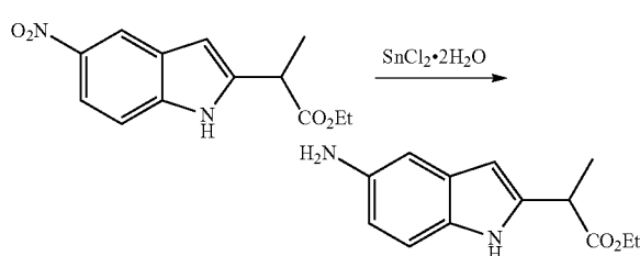
Ethyl 2-(5-amino-1H-indol-2-yl)propanoate
