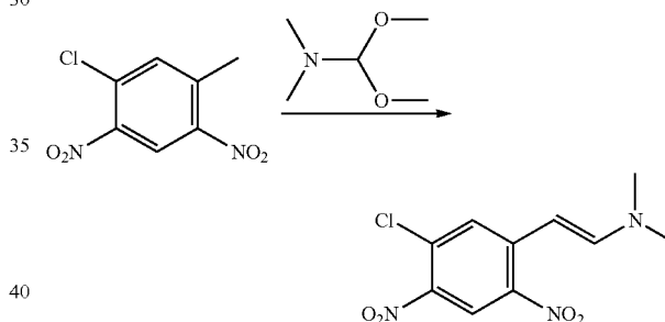
(E)-2-(5-Chloro-2,4-dinitrophenyl)-N,N-dimethylethanamine
