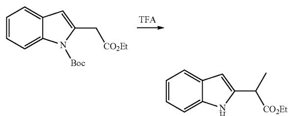
Ethyl 2-(1H-indol-2-yl)propanoate
