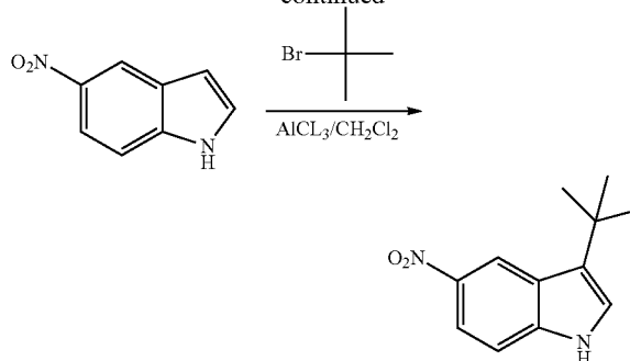
3-tert-Butyl-5-nitro-1H-indole
