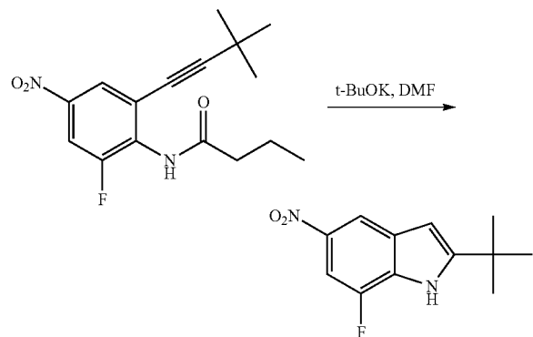
2-tert-Butyl-7-fluoro-5-nitro-1H-indole
