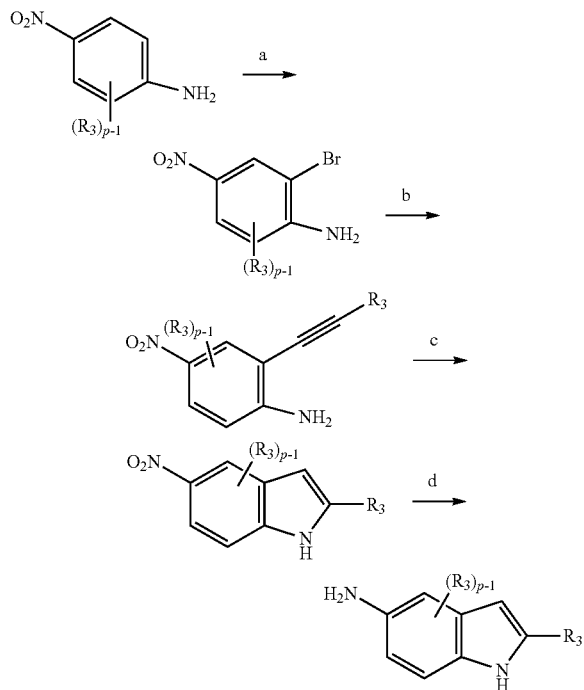
Scheme 19
