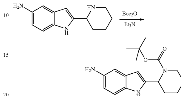
tert-Butyl 2-(5-amino-1H-indol-2-yl)piperidine-1-carboxylate
