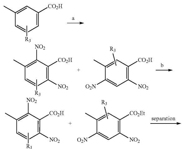
Scheme 10
