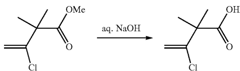
3-Chloro-2,2-dimethylbut-3-enoic acid
