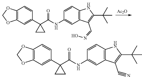
1-(Benzo[d][1,3]dioxol-5-yl)-N-(2-tert-butyl-3-cyano-1H-indol-5-yl)cyclopropanecarboxamide
