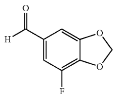
7-Fluoro-benzo[1,3]dioxole-5-carbaldehyde
