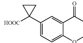
1-(4-Oxochroman-6-yl)cyclopropanecarboxylic acid
