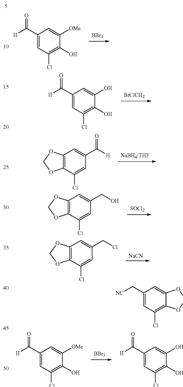
Example 18: 2-(7-Chlorobenzo[d][1,3]dioxol-5-yl)acetonitrile
