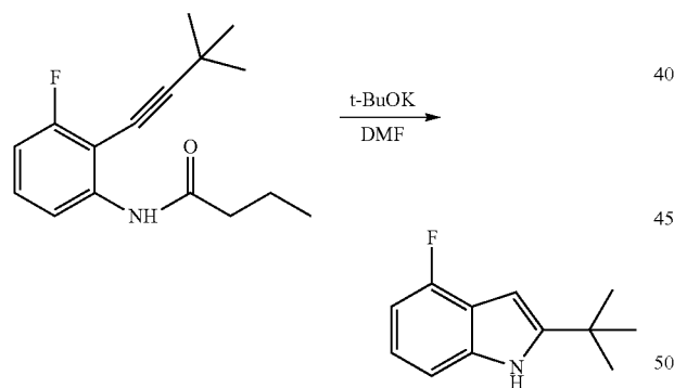
2-tert-Butyl-4-fluoro-1H-indole
