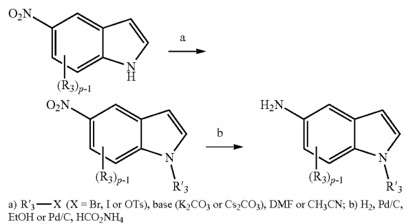
Scheme 27
