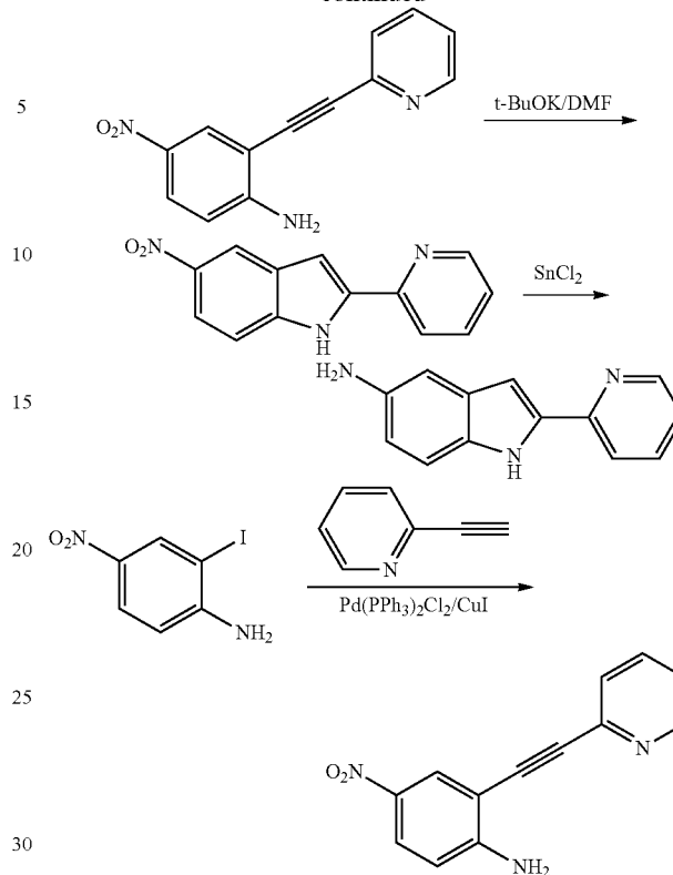
4-Nitro-2-(pyridin-2-ylethynyl)aniline
