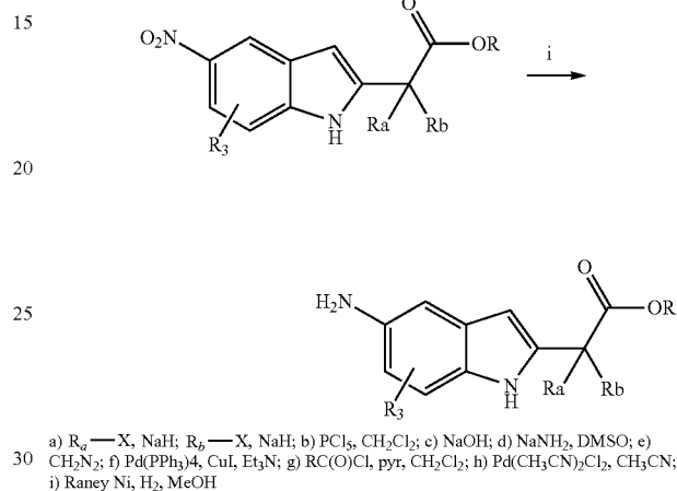
Scheme 32
