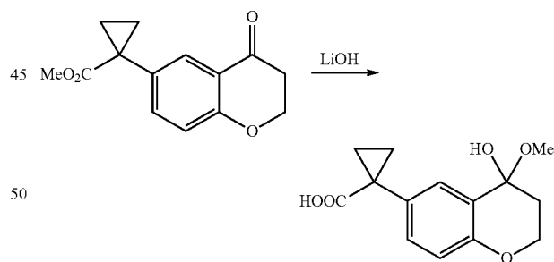
1-(4-Hydroxy-4-methoxychroman-6-yl)cyclopropanecarboxylic acid
