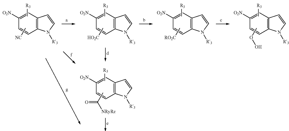
Scheme 30
