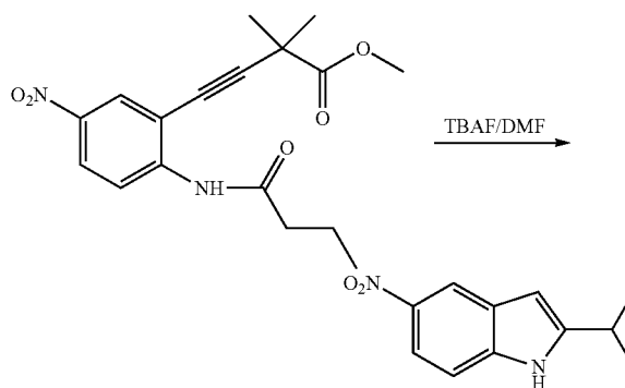
2-Isopropyl-5-nitro-1H-indole
