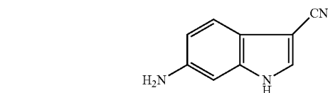
6-Amino-1H-indole-3-carbonitrile
