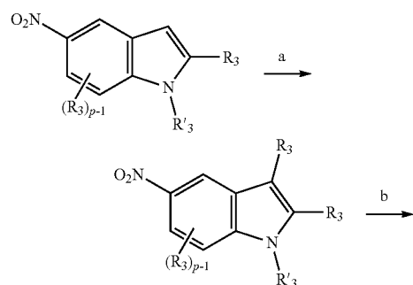
Scheme 28
