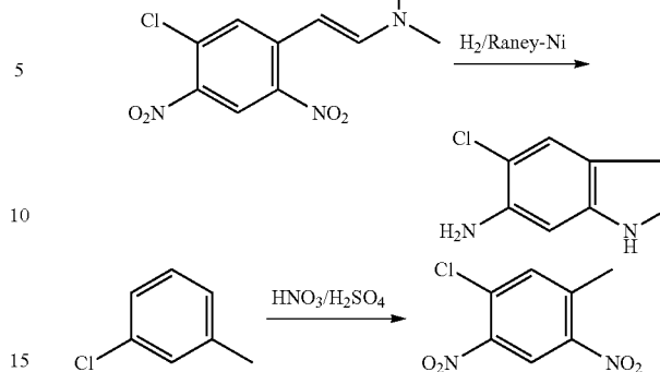
1-Chloro-5-methyl-2,4-dinitrobenzene
