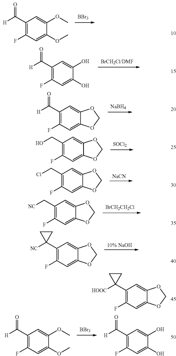
2-Fluoro-4,5-dihydroxy-benzaldehyde
