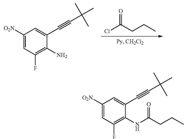
N-[2-(3,3-Dimethyl-but-1-ynyl)-6-fluoro-4-nitro-phenyl]-butyramide
