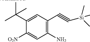
4-tert-Butyl-5-nitro-2-trimethylsilylethynyl-phenylamine
