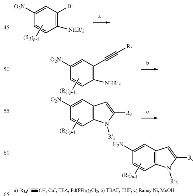
Scheme 22
