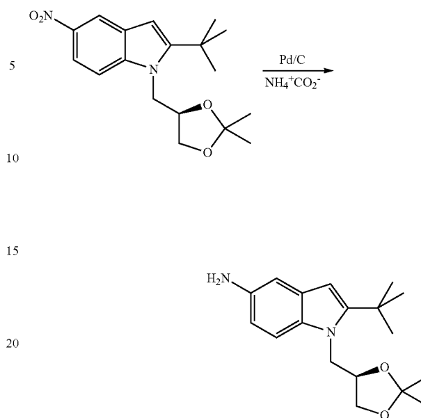
(R)-2-tert-Butyl-1-((2,2-dimethyl-1,3-dioxolan-4-yl)methyl)-5-amino-1H-indole
