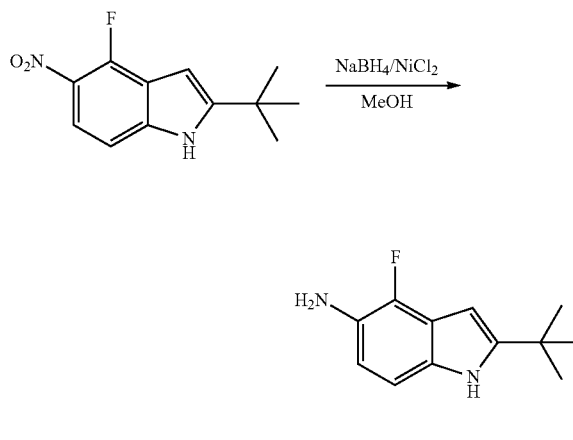
2-ter-Butyl-4-fluoro-1H-indol-5-amine
