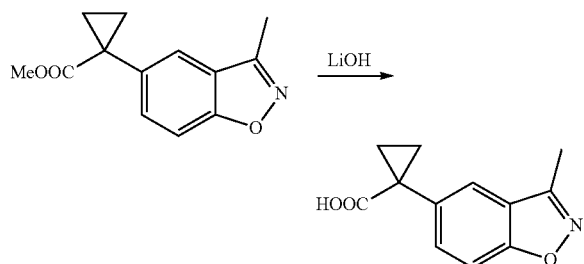
1-(3-Methylbenzo[d]isoxazol-5-yl)cyclopropanecarboxylic acid
