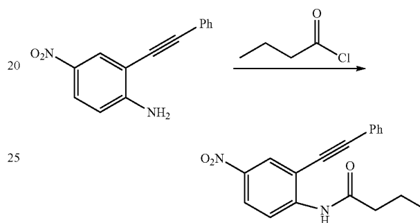
N-(2-(Phenylethynyl)phenyl)-4-nitrobutyramide
