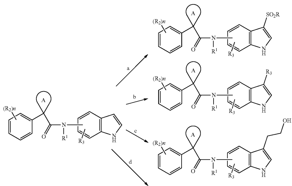
Scheme 38
