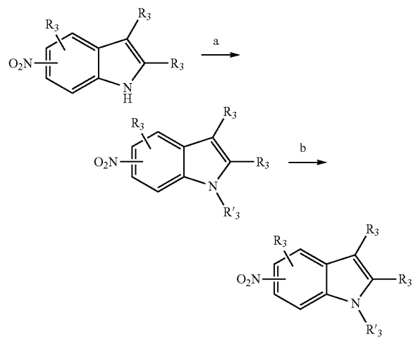
Scheme 16
