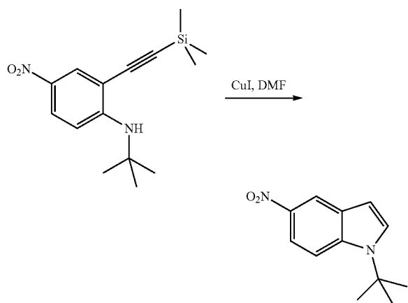
1-tert-Butyl-5-nitro-1H-indole
