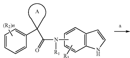
Scheme 36
