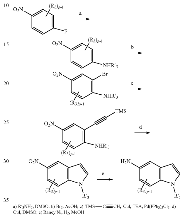
Scheme 21
