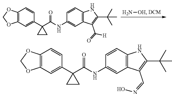
(Z)-1-(Benzo[d][1,3]dioxol-5-yl)-N-(2-tert-butyl-3-((hydroxyimino)methyl)-1H-indol-5-yl)cyclopropanecarboxamide
