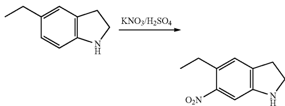
5-Ethyl-6-nitroindoline
