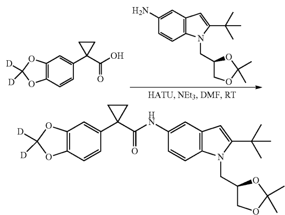
(R)—N-(2-tert-Butyl-1-((2,2-dimethyl-1,3-dioxolan-4-yl)methyl)-1H-indol-5-yl)-1-(2,2-dideuteriumbenzo[d][1,3]dioxol-5-yl)cyclopropanecarboxamide
