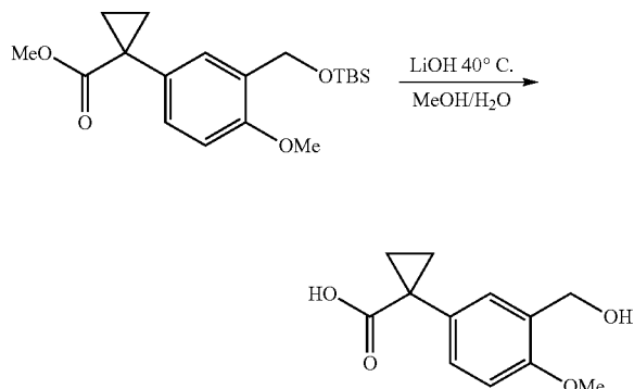
1-(3-Hydroxymethyl-4-methoxy-phenyl)-cyclopropanecarboxylic acid
