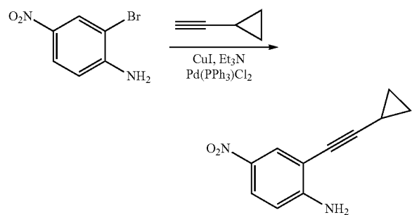
2-(Cyclopropylethynyl)-4-nitroaniline
