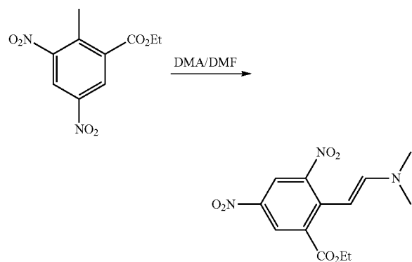
(E)-Ethyl 2-(2-(dimethylamino)vinyl)-3,5-dinitrobenzoate
