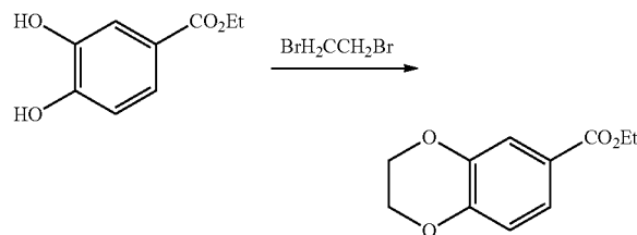
2,3-Dihydro-benzo[1,4]dioxine-6-carboxylic acid ethyl ester
