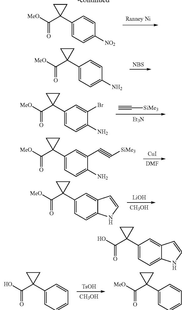
Methyl 1-phenylcyclopropanecarboxylate
