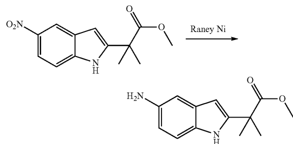
Methyl 2-(5-amino-1H-indol-2-yl)-2-methylpropanoate
