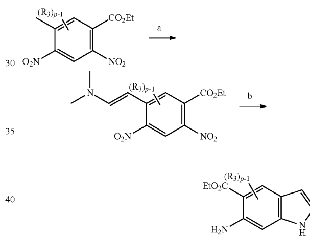
Scheme 11
