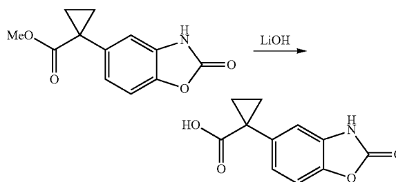
1-(2-Oxo-2,3-dihydrobenzo[d]oxazol-5-yl)cyclopropanecarboxylic acid
