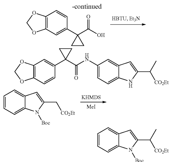
tert-Butyl 2-(1-ethoxy-1-oxopropan-2-yl)-1H-indole-1-carboxylate
