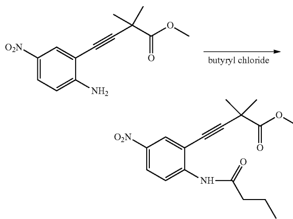
Methyl 4-(2-butylamido-5-nitrophenyl)-2,2-dimethylbut-3-ynoate
