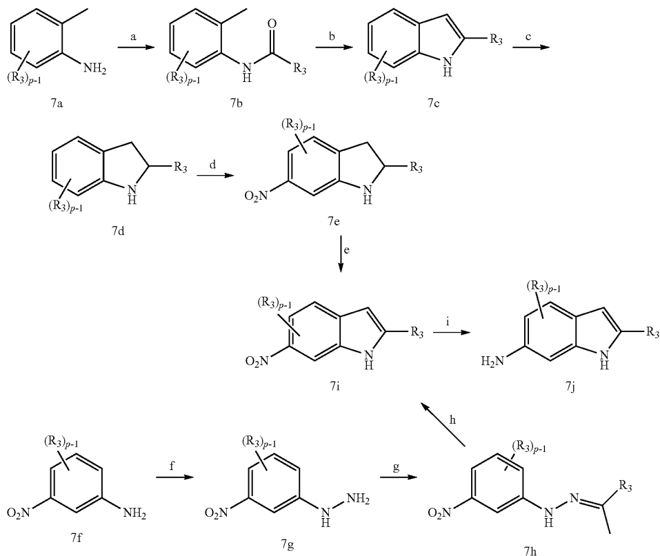
Scheme 7
