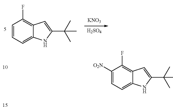
2-tert-Butyl-4-fluoro-5-nitro-1H-indole
