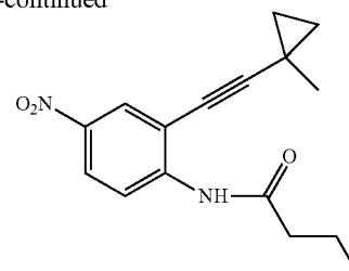
N-[2-((1-Methylcyclopropyl)ethynyl)-4-nitrophenyl]-butyramide
