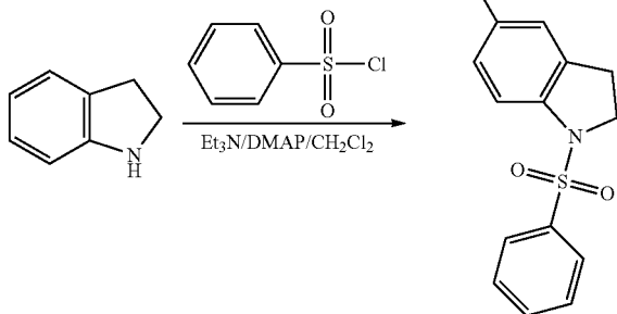
1-(Phenylsulfonyl)indoline
