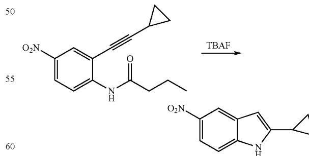
2-Cyclopropyl-5-nitro-1H-indole
