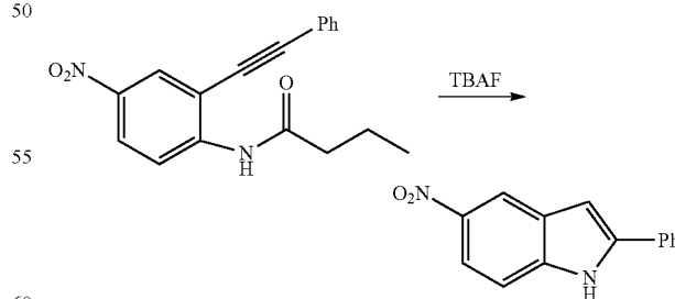
5-Nitro-2-phenyl-1H-indole
