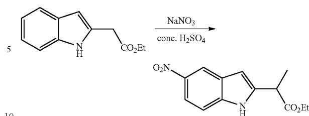
Ethyl 2-(5-nitro-1H-indol-2-yl)propanoate
