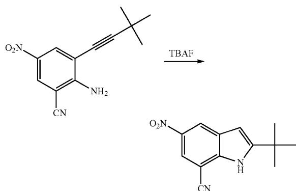
2-tert-Butyl-5-nitro-1H-indole-7-carbonitrile
