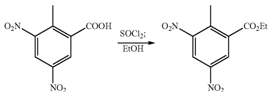
Ethyl 2-methyl-3,5-dinitrobenzoate
