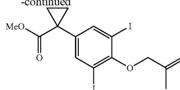
1-[3,5-Diiodo-4-(2-methyl-allyloxy)-phenyl]-cyclopropanecarboxylic acid methyl ester
