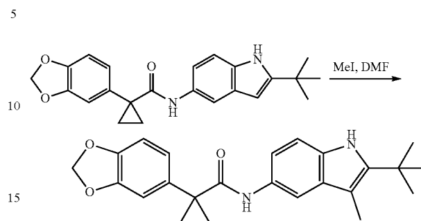
Example 85: 1-(Benzo[d][1,3]dioxol-5-yl)-N-(2-tert-butyl-3-methyl-1H-indol-5-yl)cyclopropanecarboxamide
