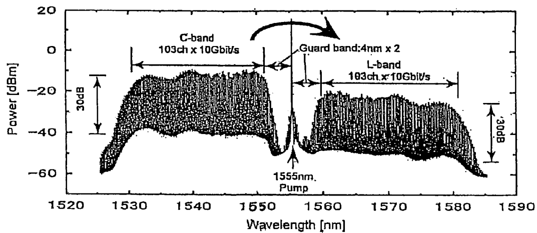
FIG.29 PPLN output spectrum
