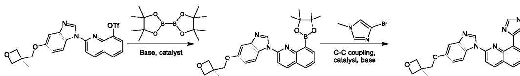
Scheme 7.
