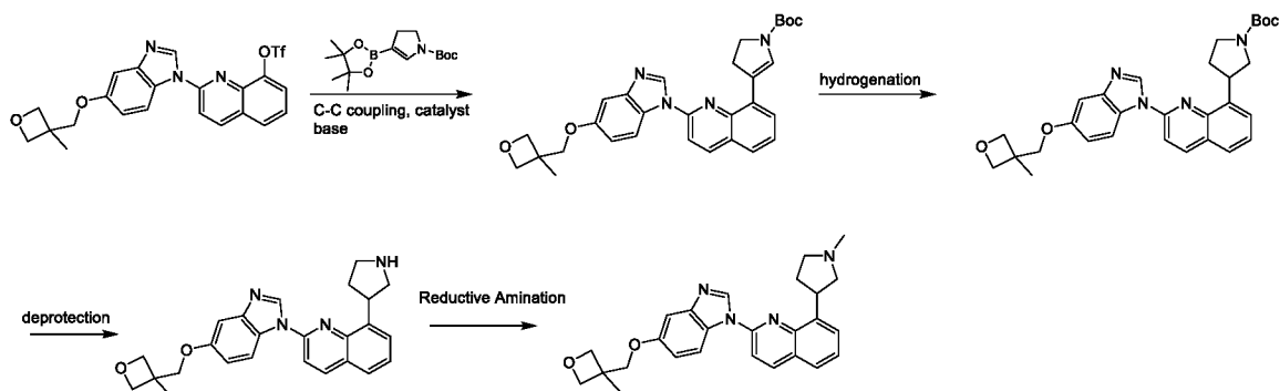
Scheme 6.
