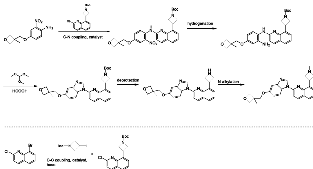
Scheme 5.
