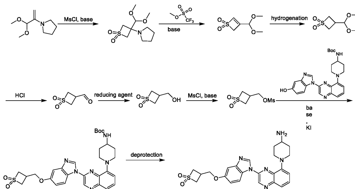
Scheme 4.
