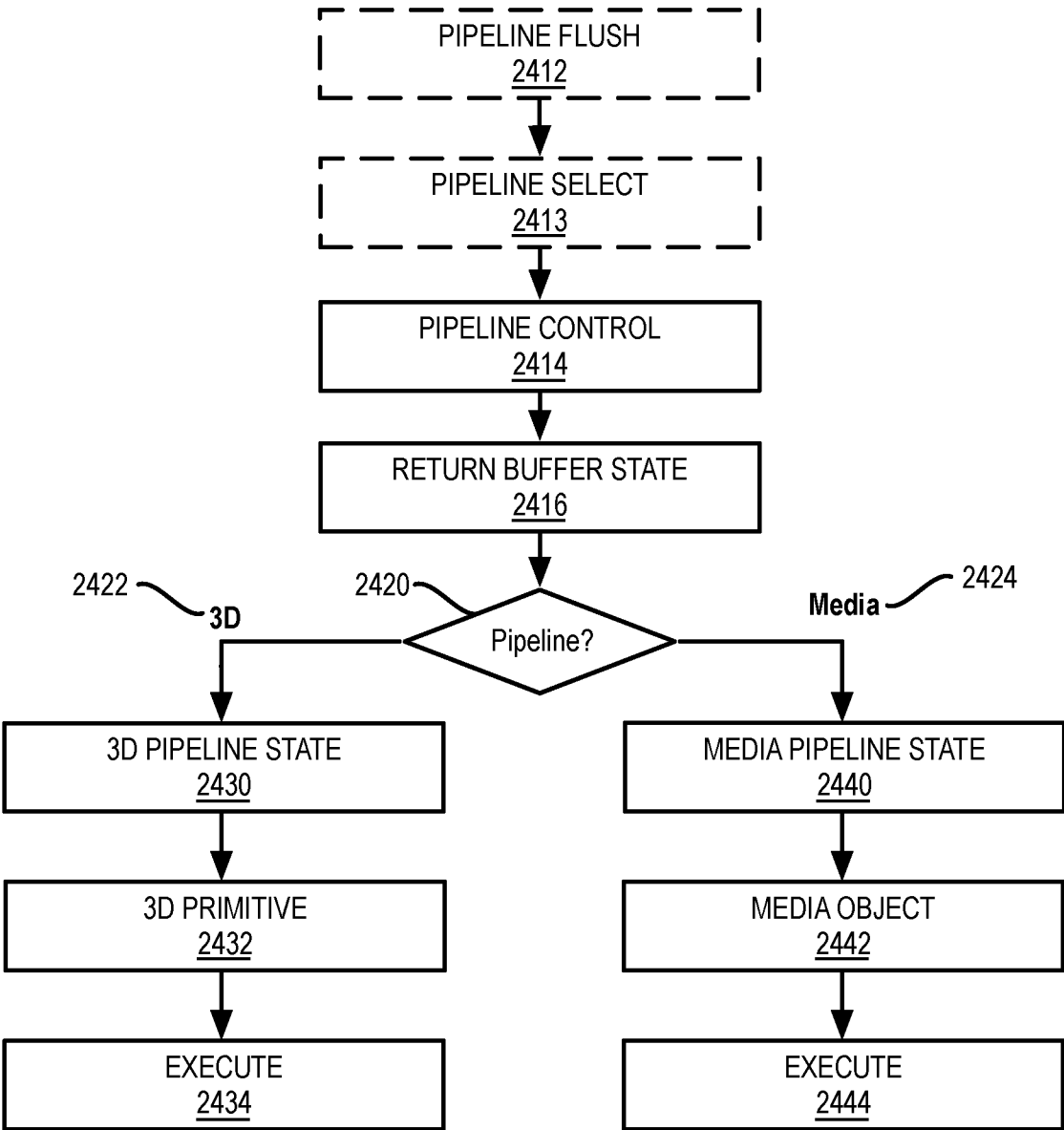
FIG. 24B GRAPHICS PROCESSOR COMMAND SEQUENCE 2410
