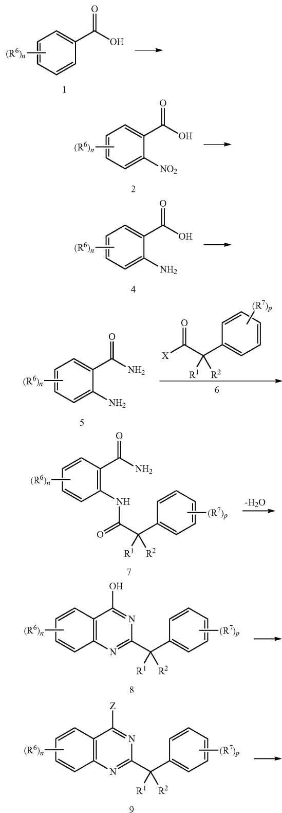
Scheme 1
