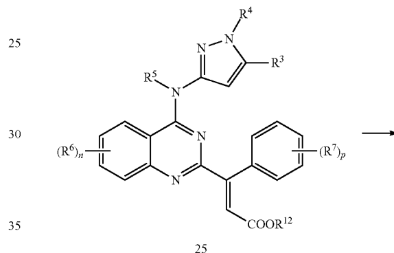
Scheme 5
