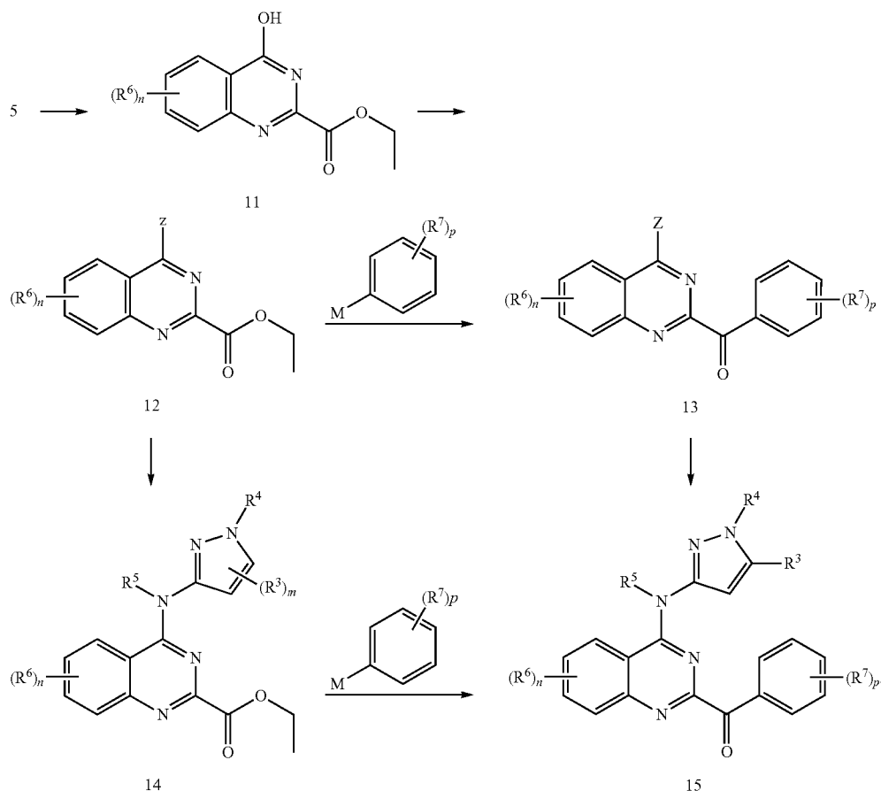
Scheme 2
