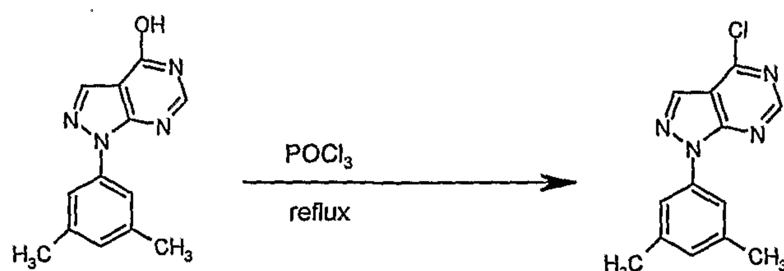
Compound No: 78
