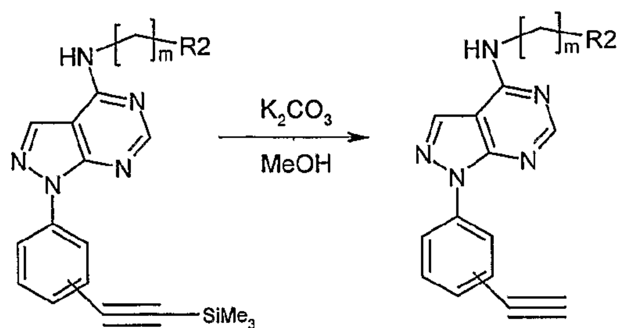
Formula-I (with acetylene group)
