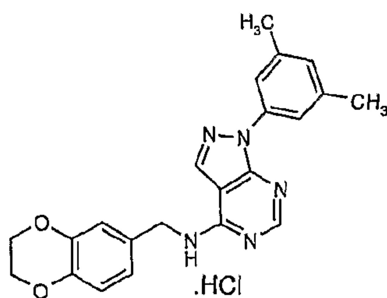
Compound NO: 49 hydrochloride
