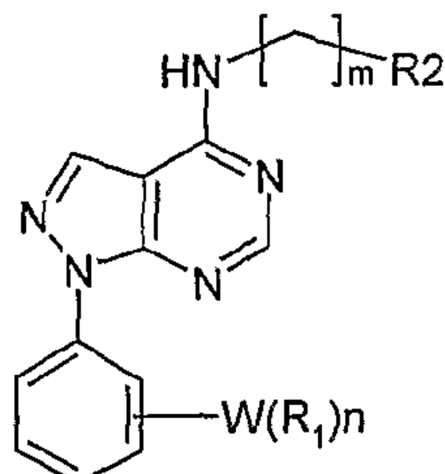
Formula-I
