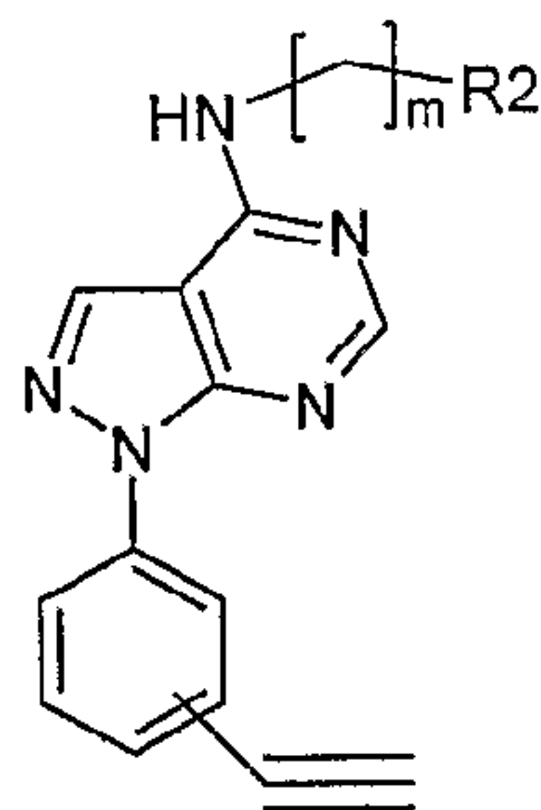
Formula-I (with acetylene group)
