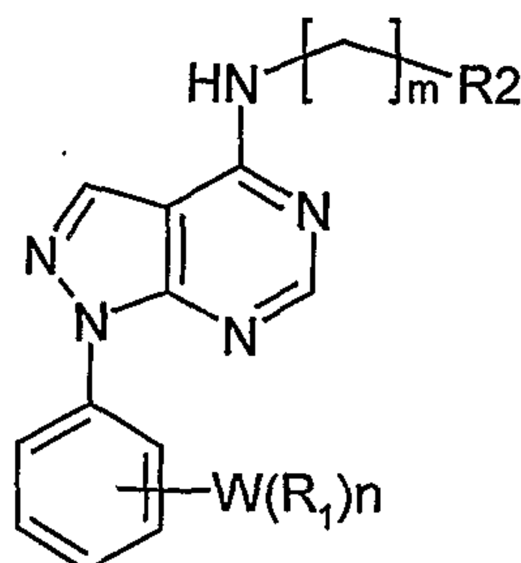
Formula-I
