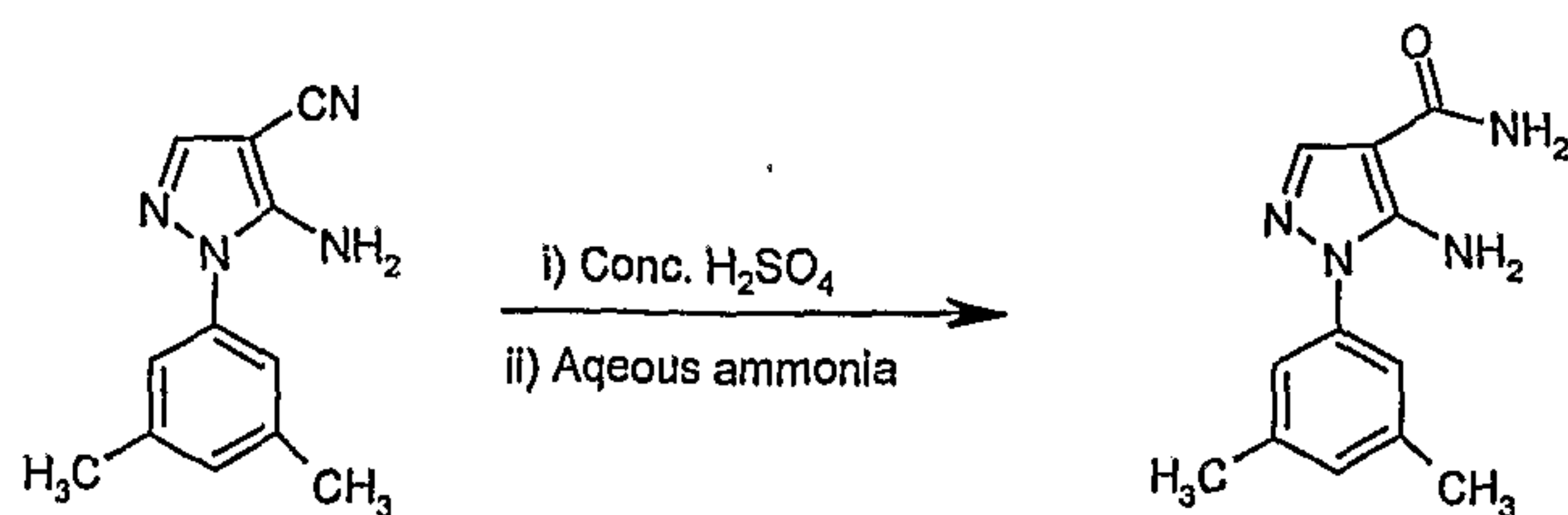
Compound No: 77
