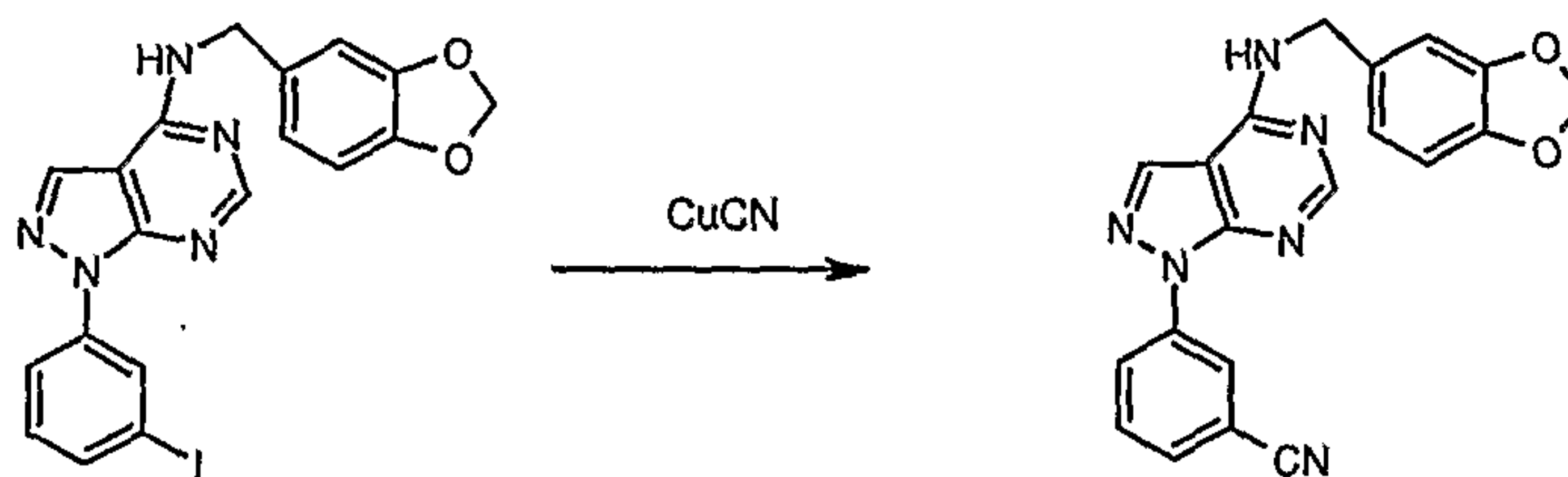
Compound No: 30
