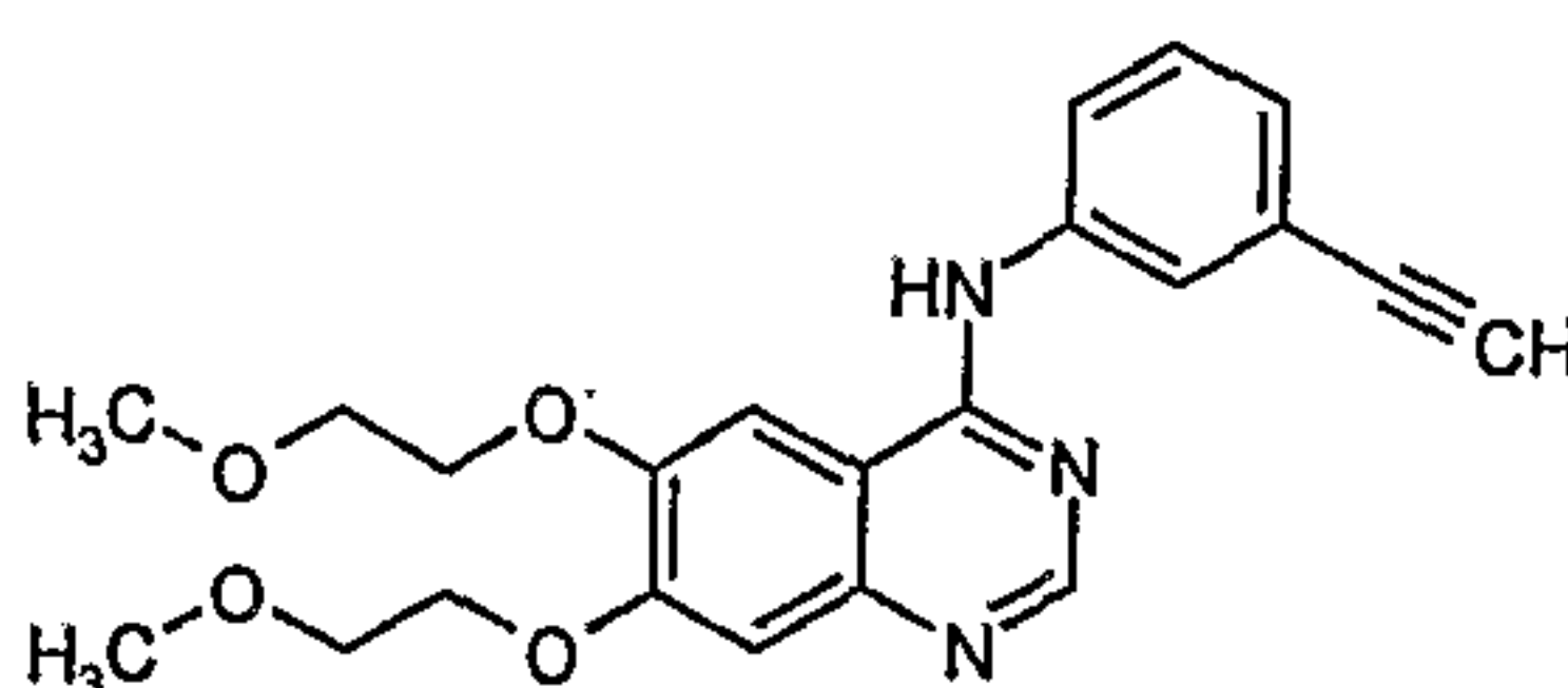
Formula-III
