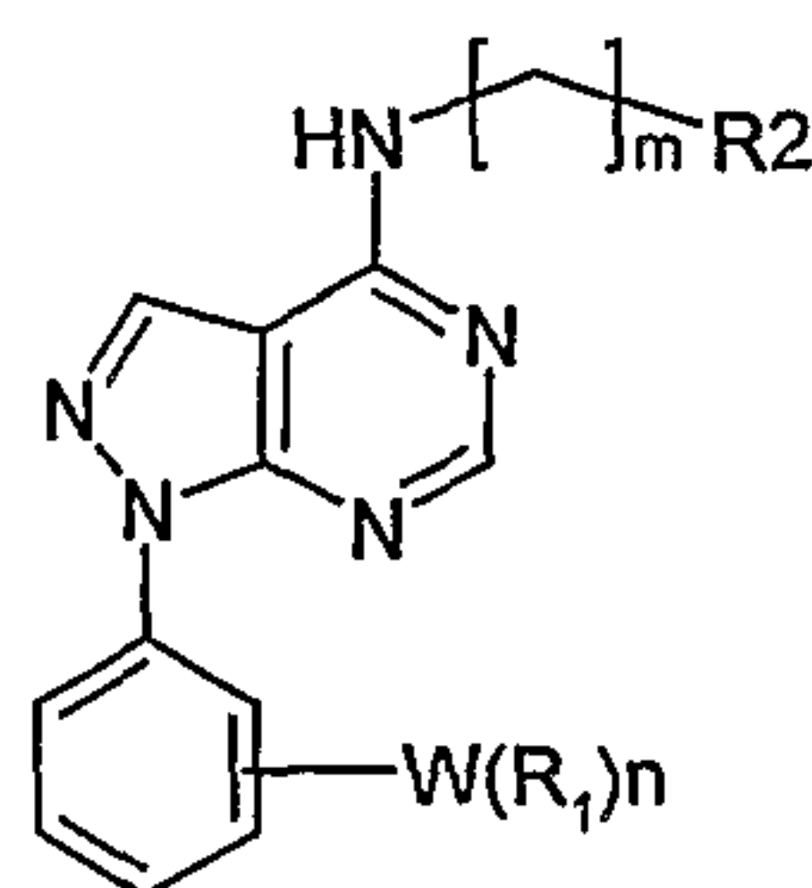
Formula-I
