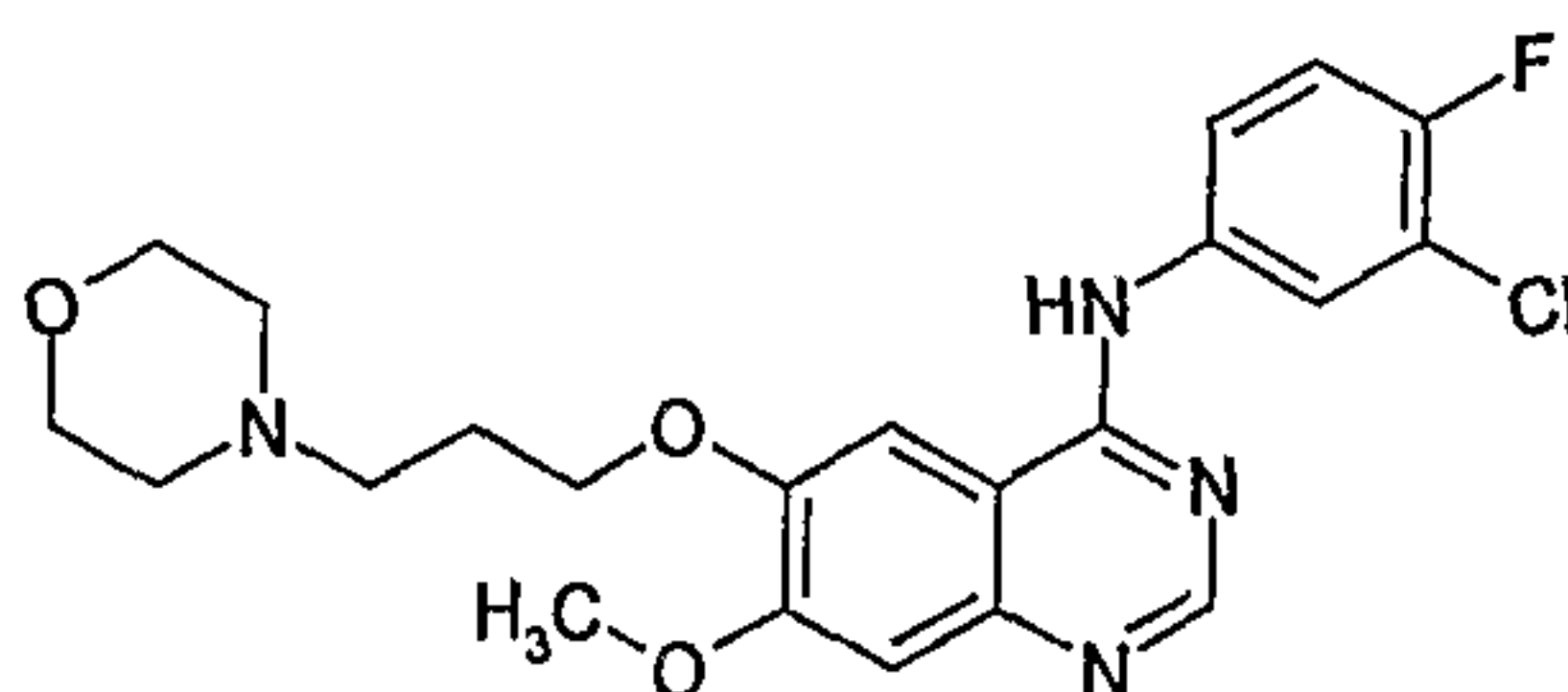
Formula-II
