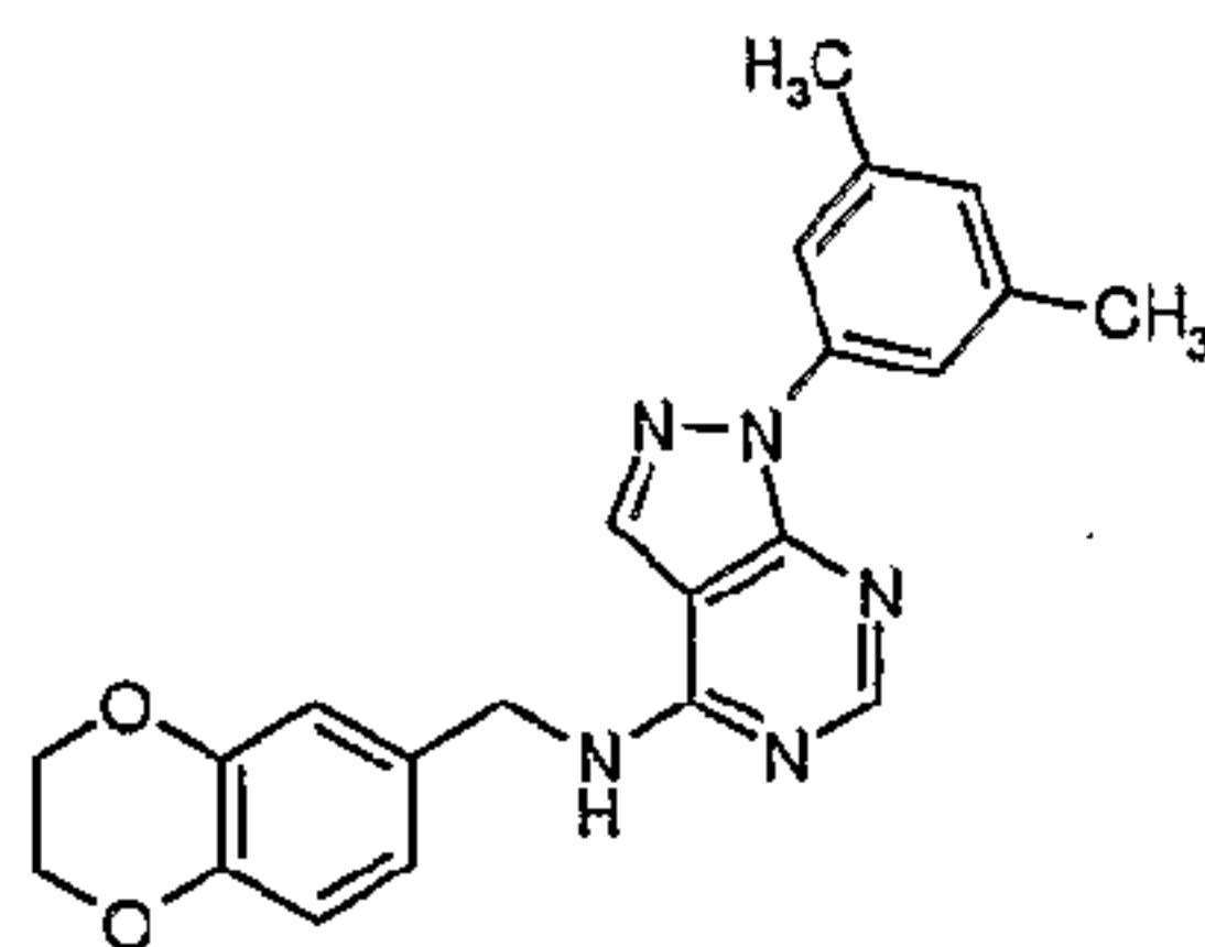
Compound NO: 49
