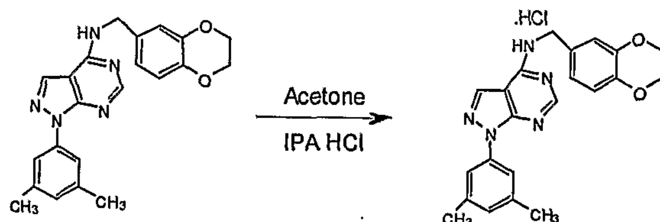
Compound No: 49
