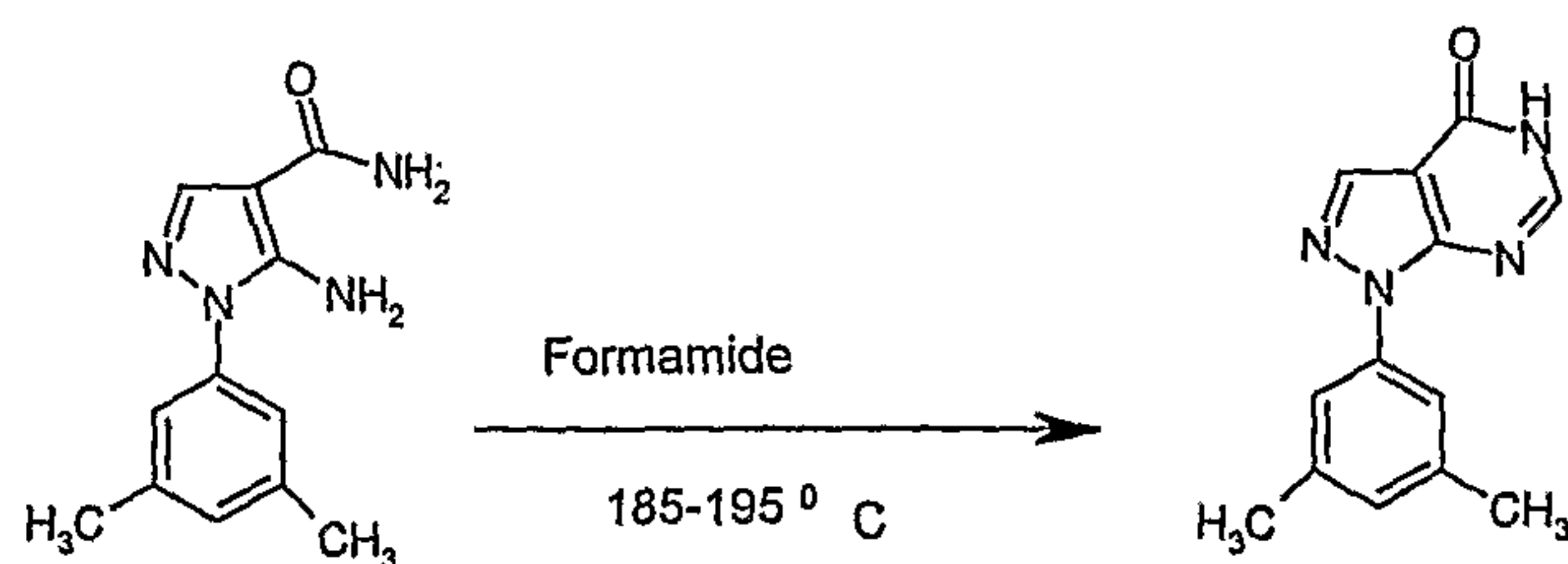
Compound No: 77
