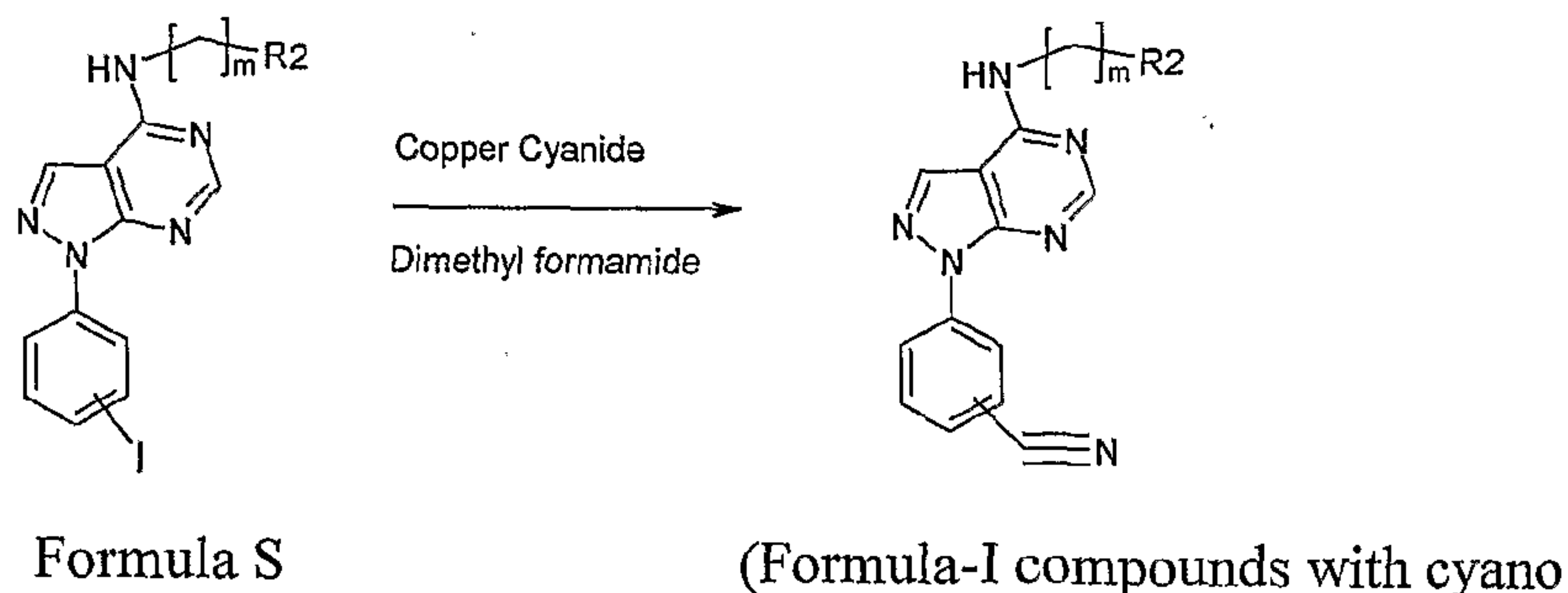
Scheme-III
