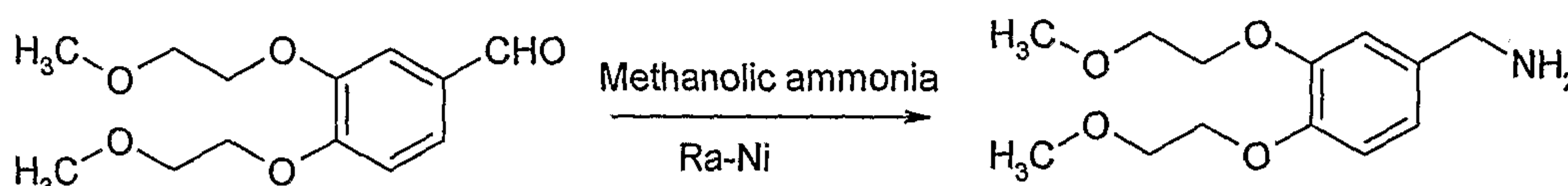
Compound No: 86
