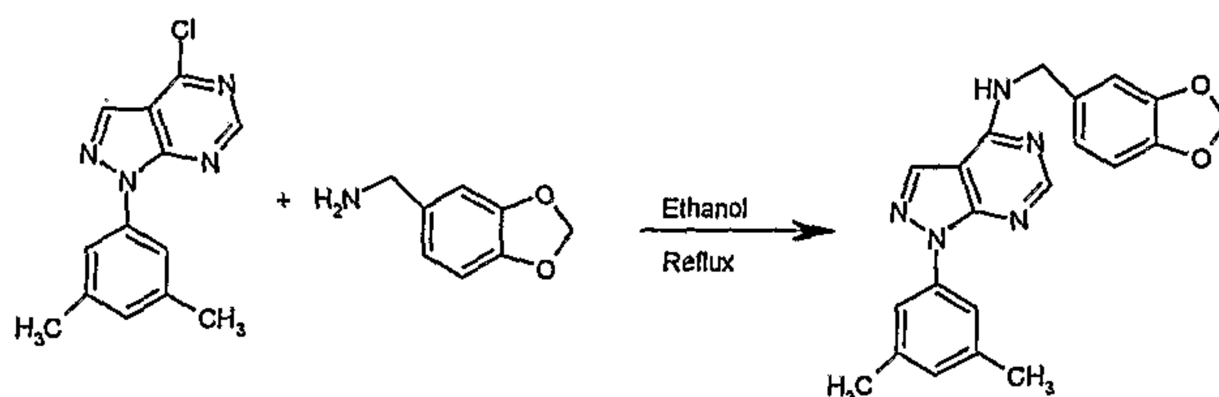
Compound No: 79
