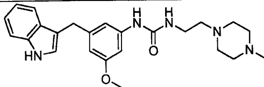
1-(3-((1H-indol-3-yl)methyl)-5-methoxyphenyl)-3-(2-(4-methylpiperazin-1-yl)ethyl)urea;
