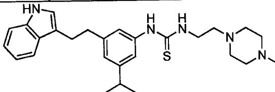
1-(3-(2-(1H-indol-3-yl)ethyl)-5-isopropylphenyl)-3-(2-(4-methylpiperazin-1-yl)ethyl)thiourea;
