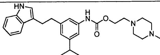
2-(4-methylpiperazin-1-yl)ethyl (3-(2-(1H-indol-3-yl)ethyl)-5-isopropylphenyl)carbamate;
