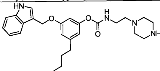
3-((1H-indol-3-yl)methoxy)-5-butylphenyl (2-(piperazin-1-yl)ethyl)carbamate;
