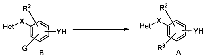
Scheme B
