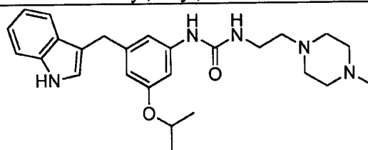
1-(3-((1H-indol-3-yl)methyl)-5-isopropoxyphenyl)-3-(2-(4-methylpiperazin-1-yl)ethyl)urea;
