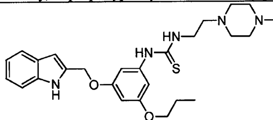
1-(3-((1H-indol-2-yl)methoxy)-5-propoxyphenyl)-3-(2-(4-methylpiperazin-1-yl)ethyl)thiourea; and
