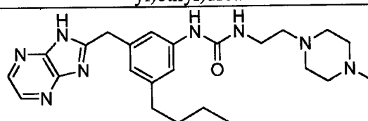
1-(3-((1H-imidazo[4,5-b]pyrazin-2-yl)methyl)-5-butylphenyl)-3-(2-(4-methylpiperazin-1-yl)ethyl)urea;
