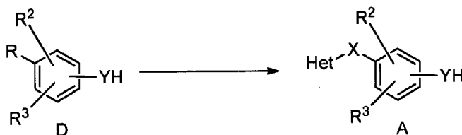
Scheme D
