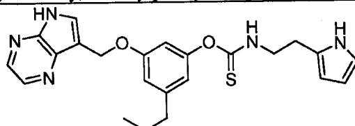
O-(3-((5H-pyrrolo[2,3-b]pyrazin-7-yl)methoxy)-5-propylphenyl) (2-(1H-pyrrol-2-yl)ethyl)carbamothioate;
