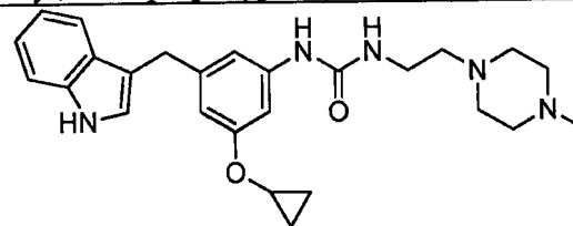
1-(3-((1H-indol-3-yl)methyl)-5-cyclopropoxyphenyl)-3-(2-(4-methylpiperazin-1-yl)ethyl)urea;
