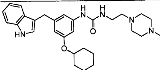
1-(3-((1H-indol-3-yl)methyl)-5-(cyclohexyloxy)phenyl)-3-(2-(4-methylpiperazin-1-yl)ethyl)urea;
