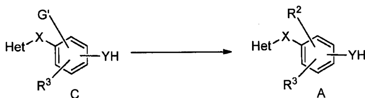
Scheme C
