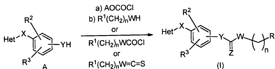
Scheme A
