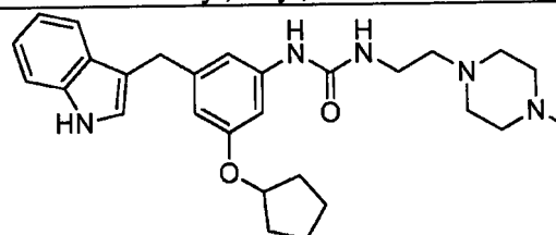
1-(3-((1H-indol-3-yl)methyl)-5-(cyclopentyloxy)phenyl)-3-(2-(4-methylpiperazin-1-yl)ethyl)urea;
