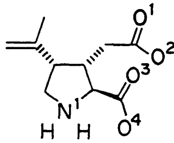
Pharmacophore Model
