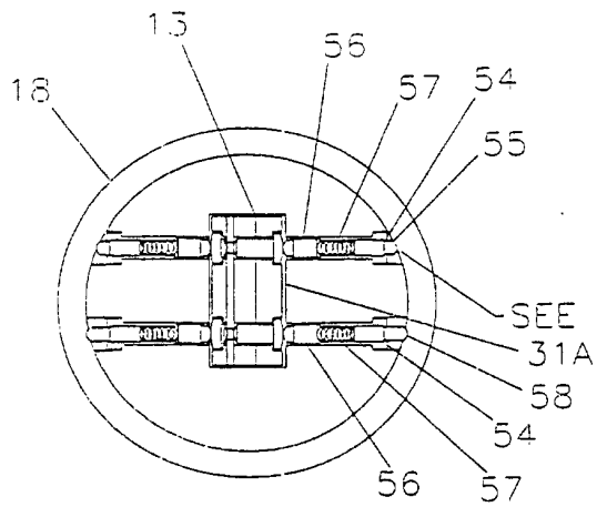
SECTION B-B FIGURE 7
