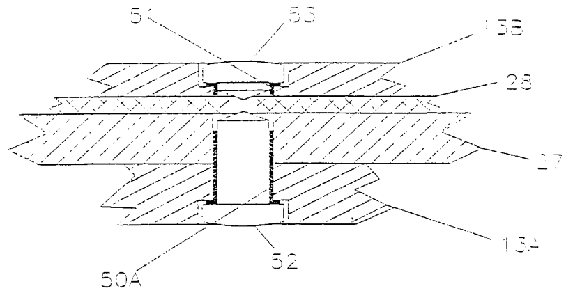
SECTION A-A FIGURE 6
