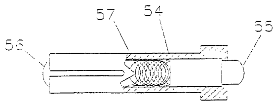
CONTACT DETAIL FIGURE 8
