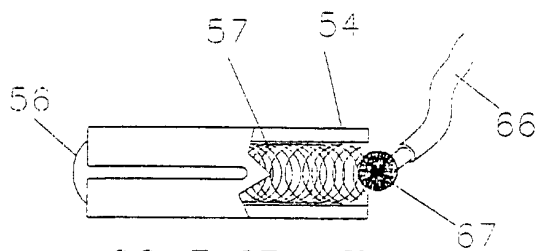
CONTACT DETAIL FIG. 14
