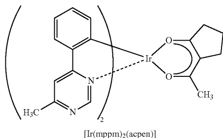
[Ir(mppm) 2 (acpen)]
