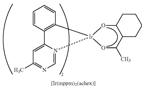
[\text{Ir}(\text{mppm})_2(\text{achex})]
