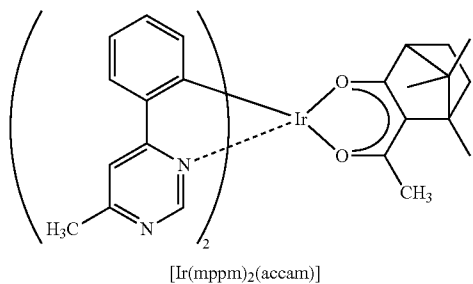
[Ir(mppm) 2 (accam)]
