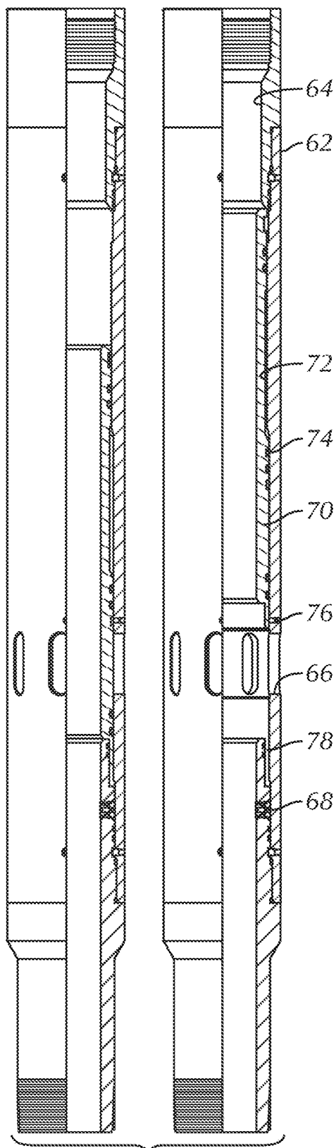
FIG. 2D (Prior Art)
