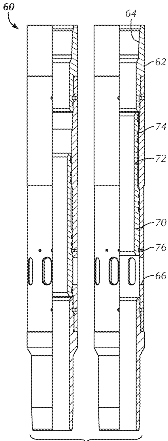
FIG. 2C (Prior Art)
