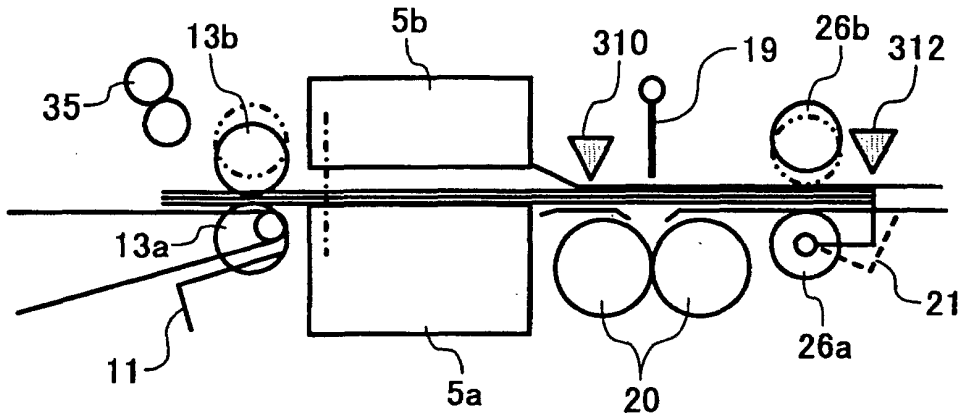
FIG. 10C BUNDLE FEED → CONTACTING
