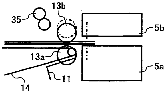
FIG. 9C STAPLER MOVEMENT
