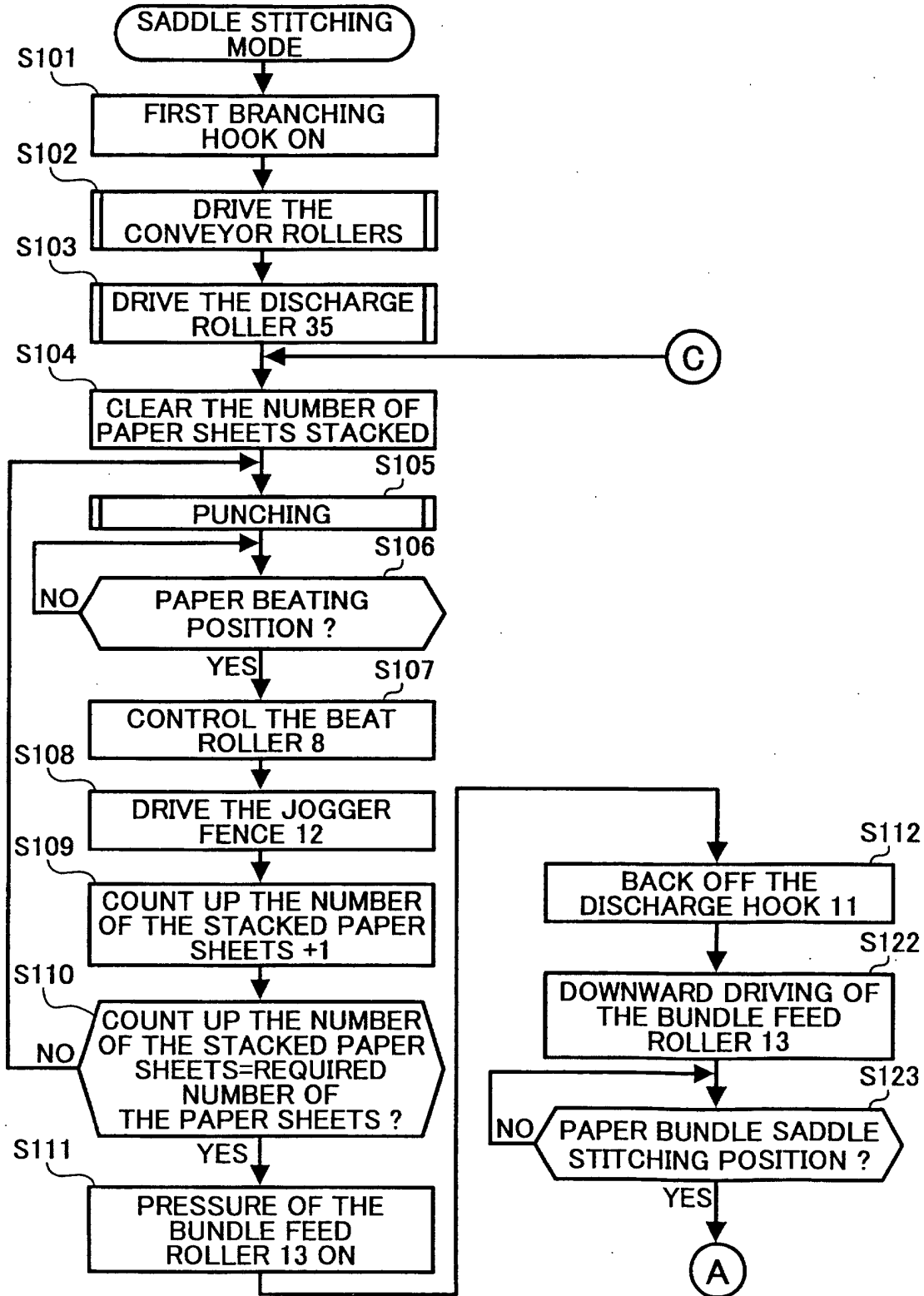
FIG. 20A SADDLE STITCHING MODE
