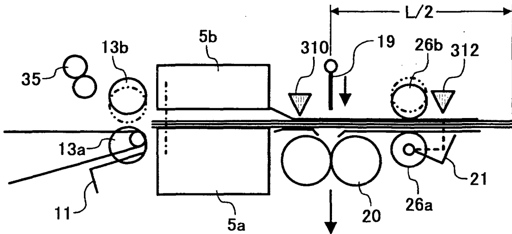
FIG. 10D FOLDING
