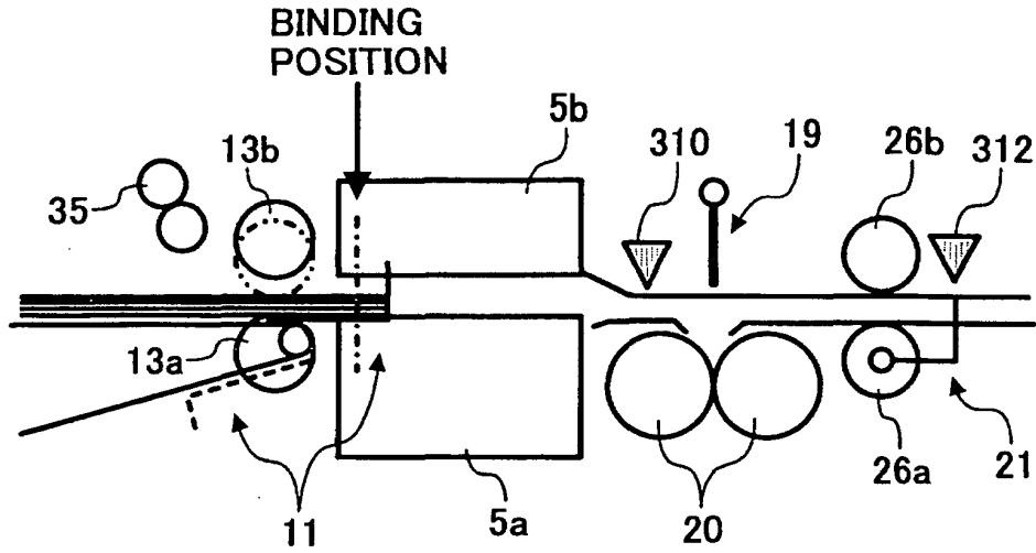
FIG. 10A ADJUSTMENT
