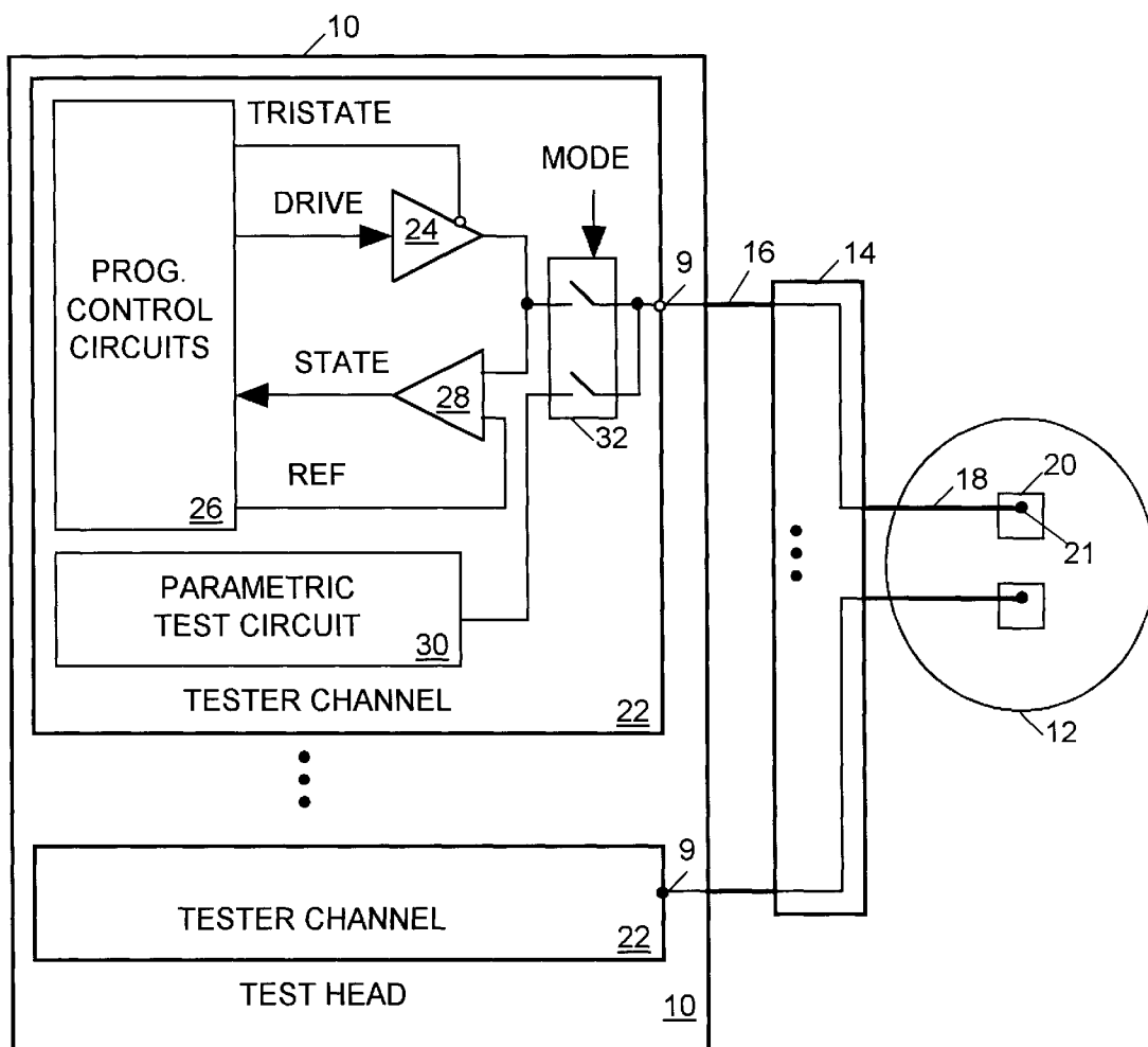
FIG. 3 (PRIOR ART)
