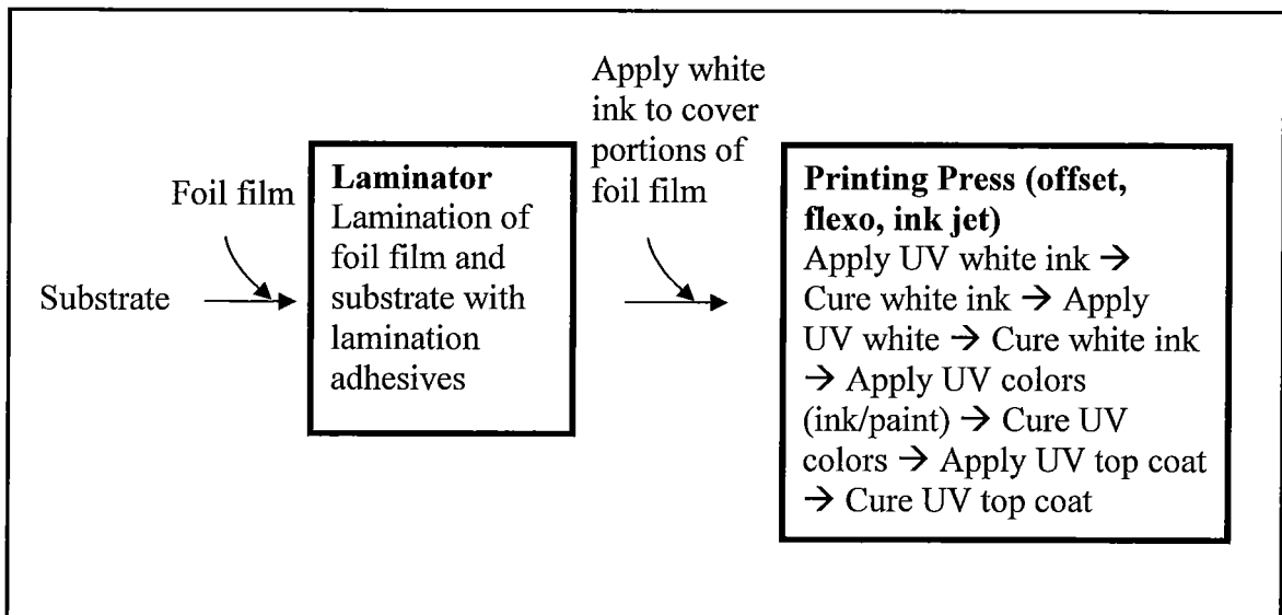
Figure 3B: Process Flow for Conventional Lamination
