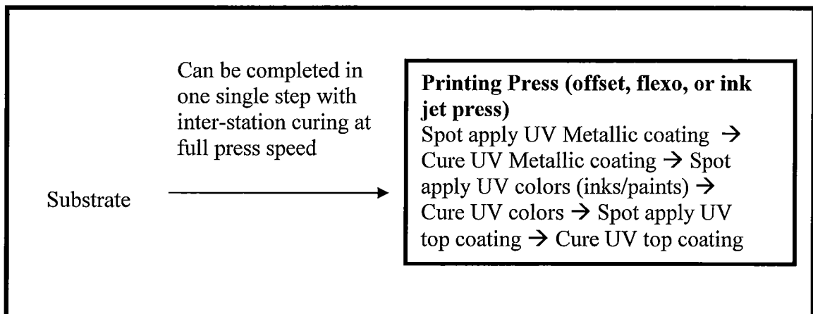
Figure 1C: Process Flow for UV Metallic Coating
