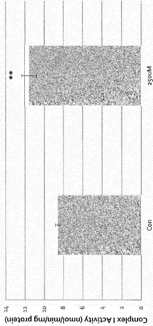
Effect of 250 \mu M C10 for 6 Days on Complex I Activity
