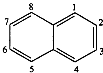
EQUATION 1
