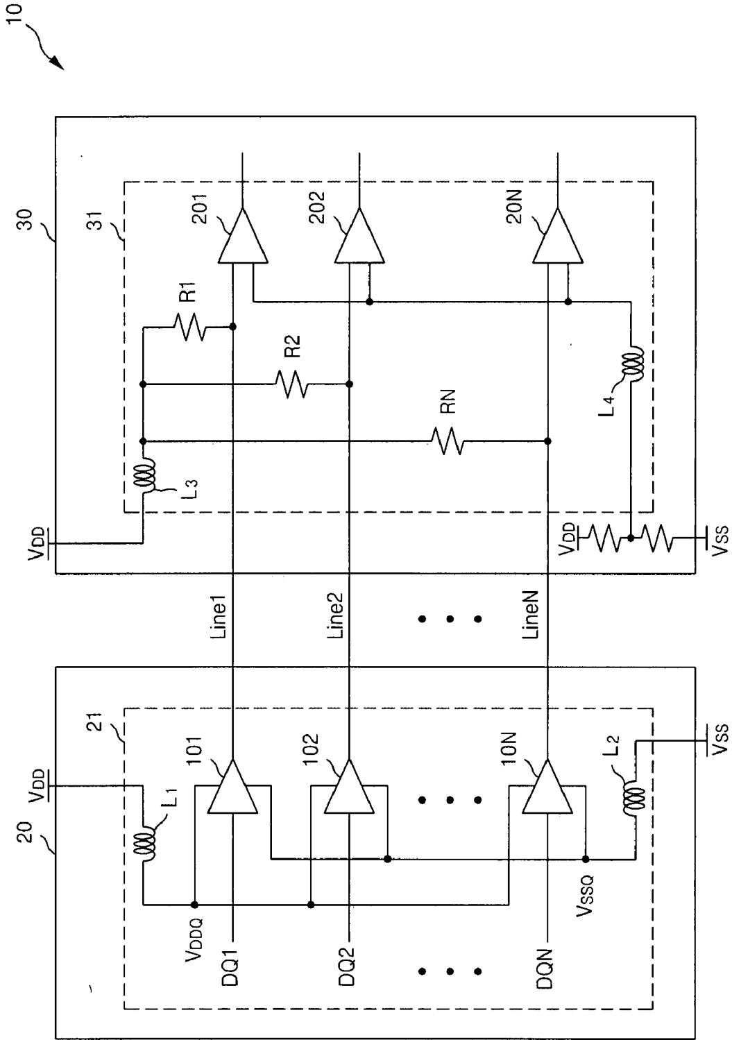
FIG. 1 (CONVENTIONAL ART)
