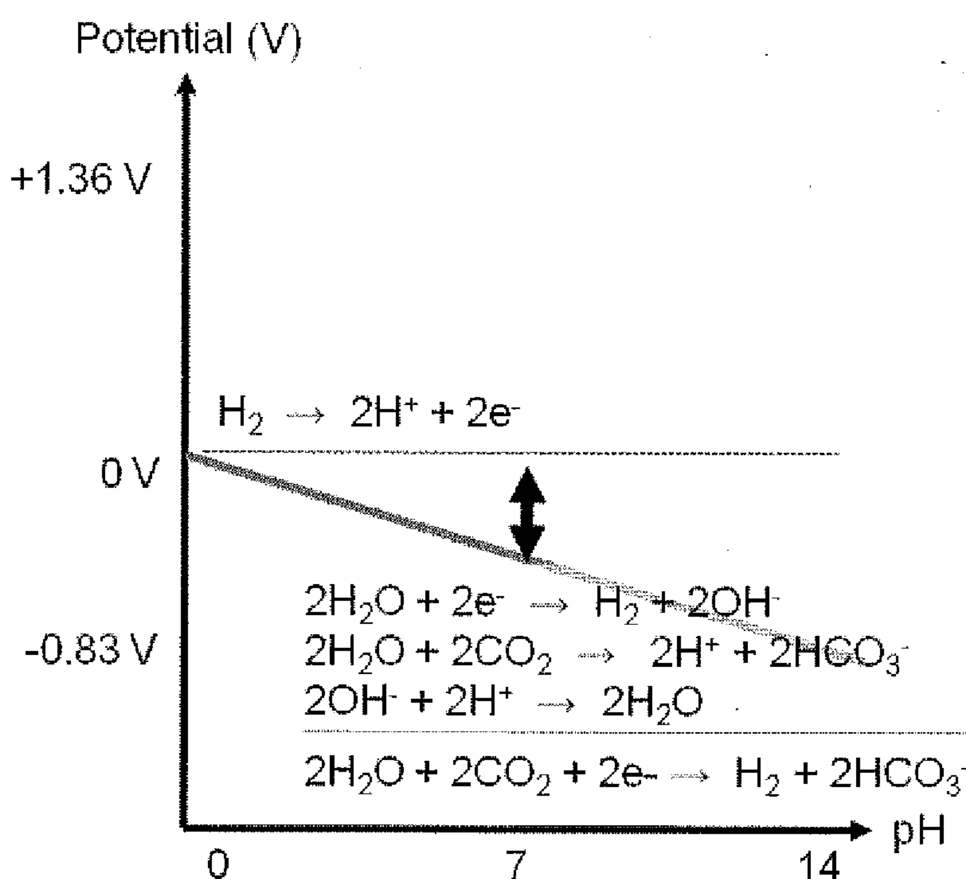
Scenario 1: Bicarbonate Ion Generation in the Cathode Electrolyte
