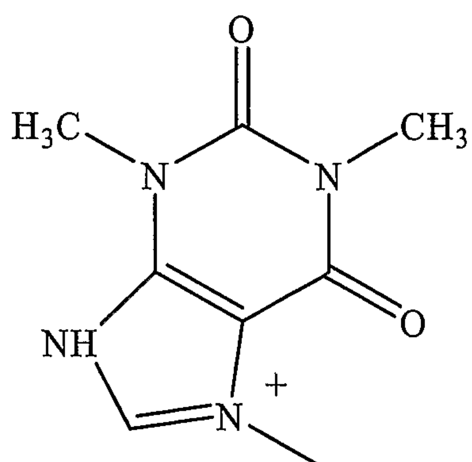
(theophylline)
