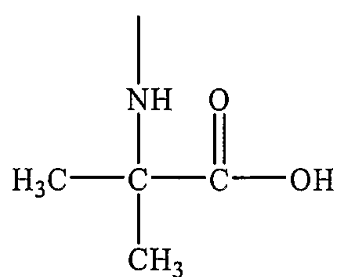
(alpha-aminoisobutyric acid)
