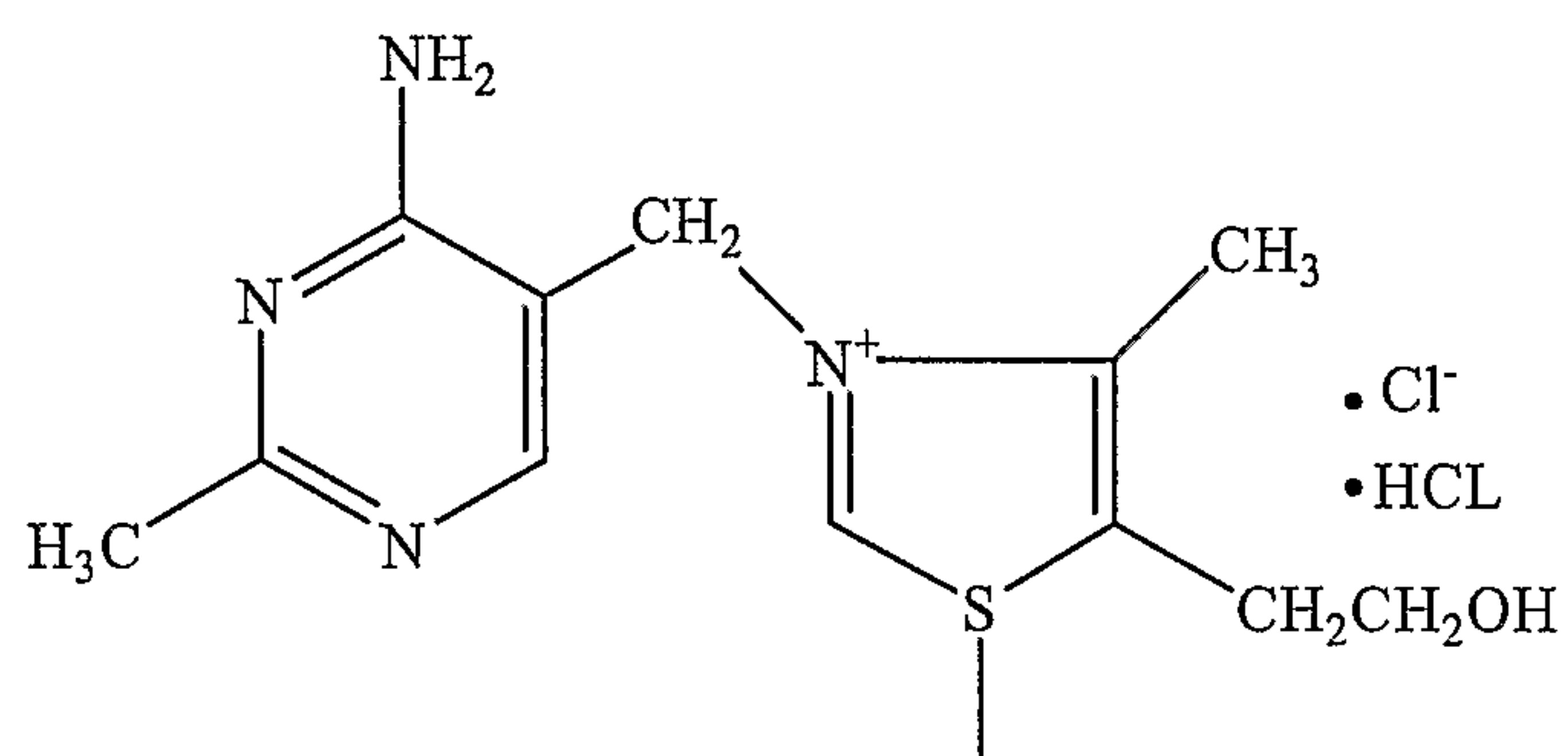
(thiamine hydrochloride)
