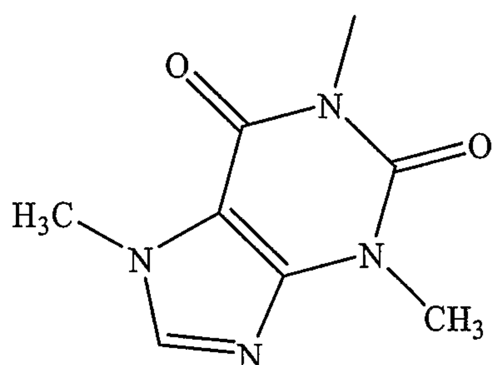
(theobromine)
