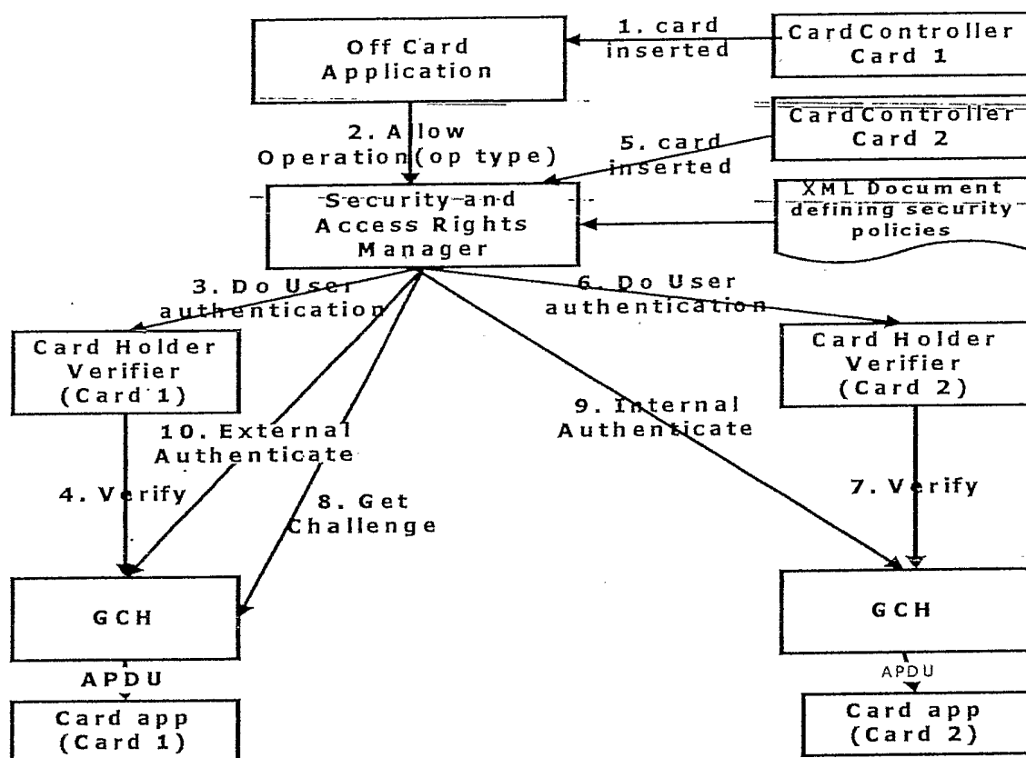
Figure 3 - Typical Authentication flow of control
