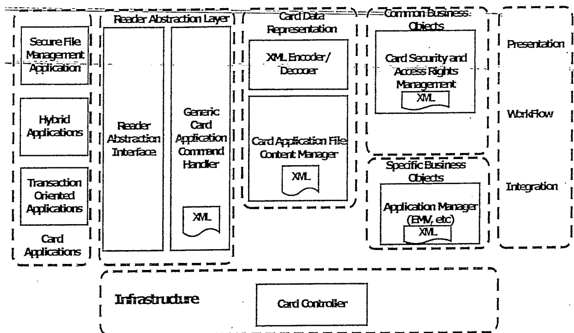
Figure 1 - Component Architecture
