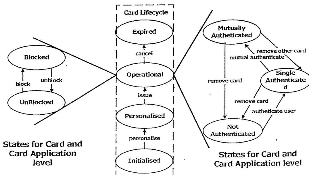
Figure 2 - Card/Card Application Operational States
