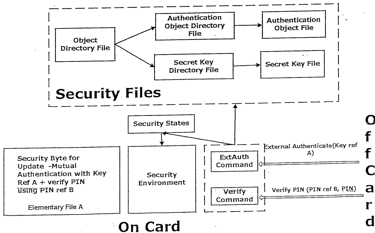
Figure 6 - Handling security for updating a file
