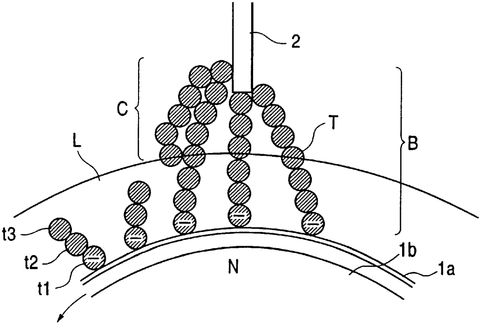
FIG. 7 PRIOR ART
