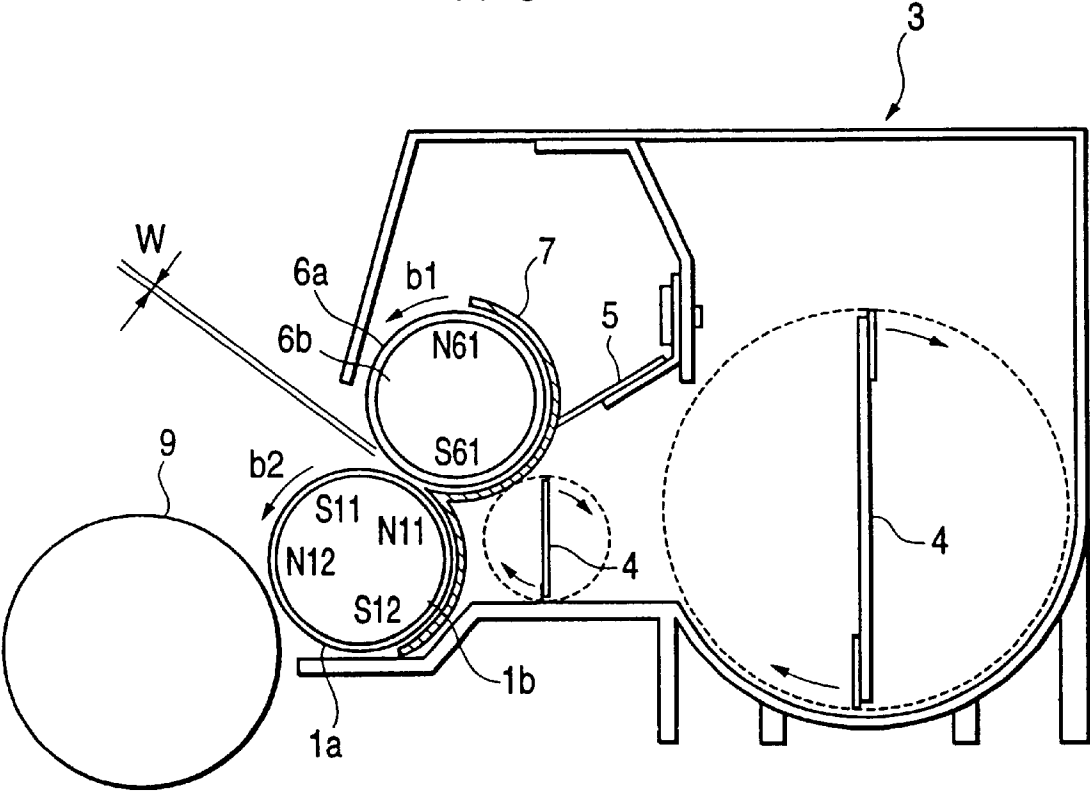
FIG. 8 PRIOR ART
