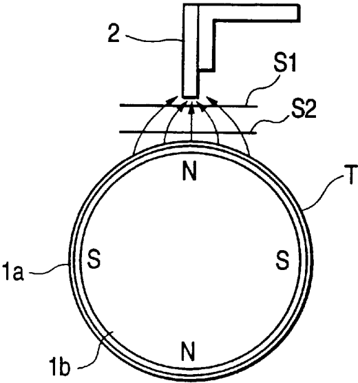
FIG. 6 PRIOR ART
