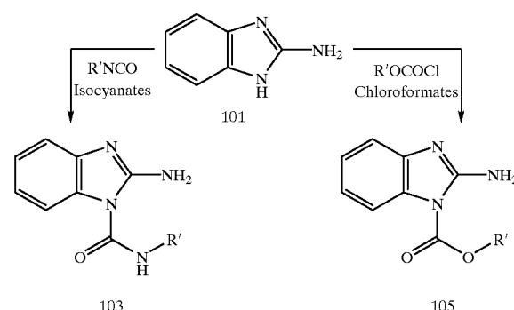
Reaction Scheme 1
