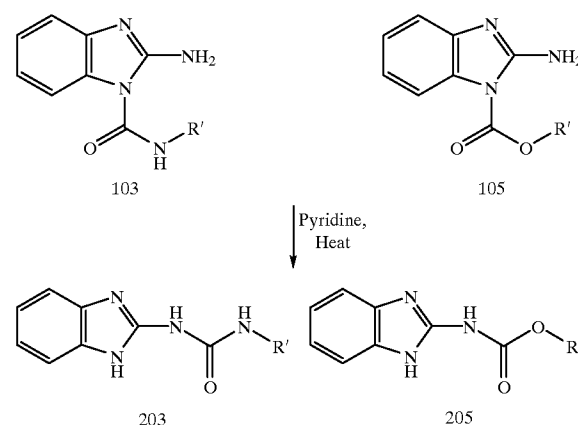
Reaction Scheme 2
