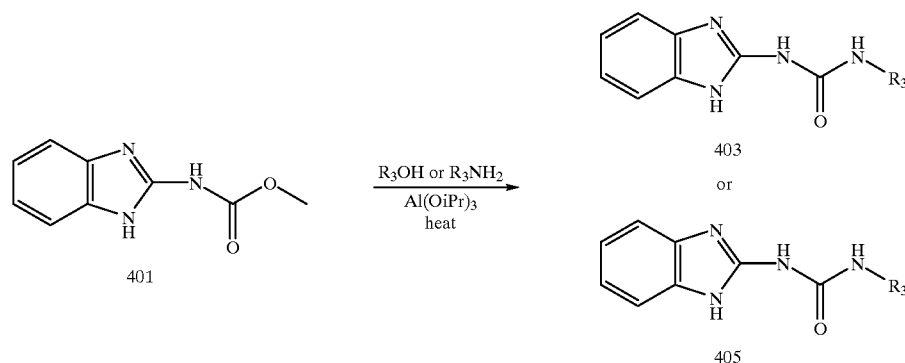
Reaction Scheme 4
