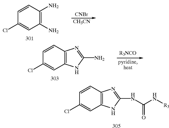
Reaction Scheme 3
