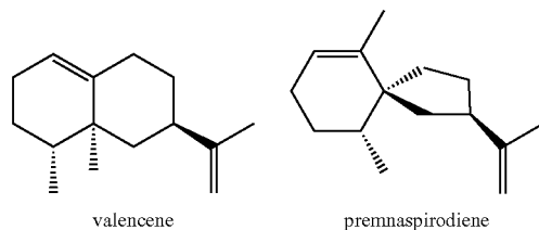
Scheme 3. Structures of valencene and premnaspirodiane.
