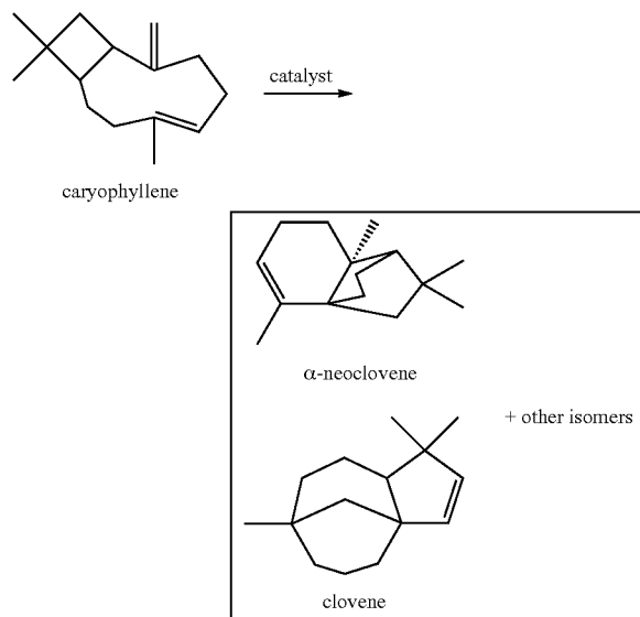
Scheme 2. Isomerization of caryophyllene with heterogeneous acid catalyst.
