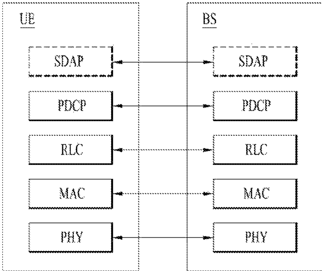
(a) User Plane Protocol Stack
