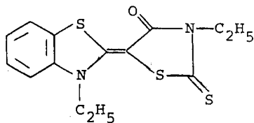
Apocyanine
