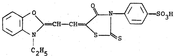
Merocyanine
