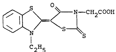
Apocyanine
