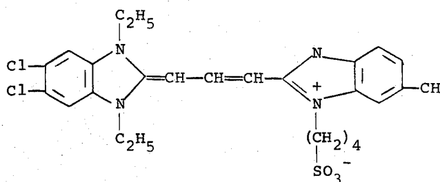
Benzimidazolocarbo-cyanine
