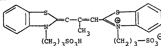
Thiocarbocyanine
