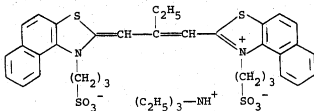
Thiocarbocyanine
