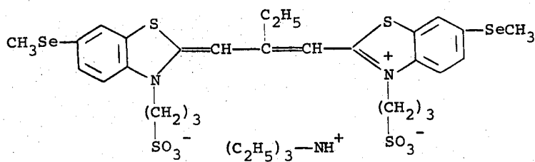
Thiocarbocyanine
