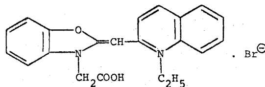
Oxa-2'-cyanine
