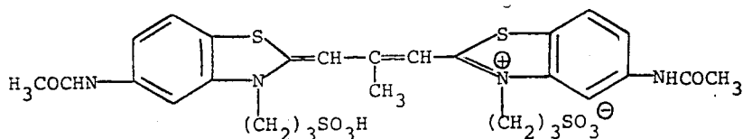
Thiacarbocyanine
