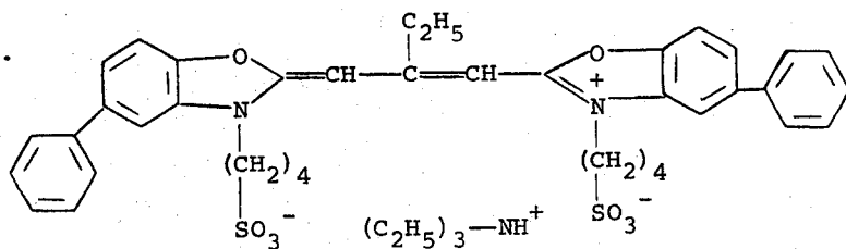
Oxacarbocyanine
