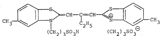
Thiacarbocyanine
