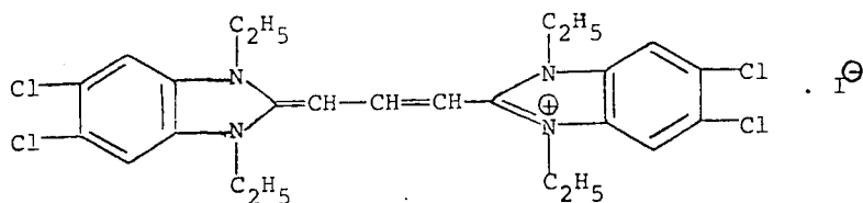
Benzimidazolocarbyanine
