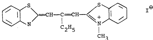
Thiacarbocyanine
