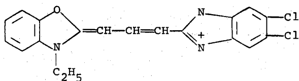
Benzimidazol-oxacarbocyanine
