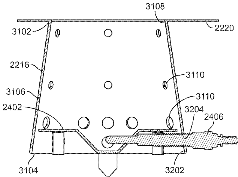
SECTION F-F
