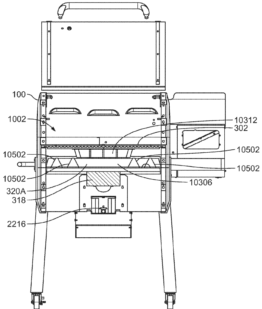
SECTION W-W FIG. 106
