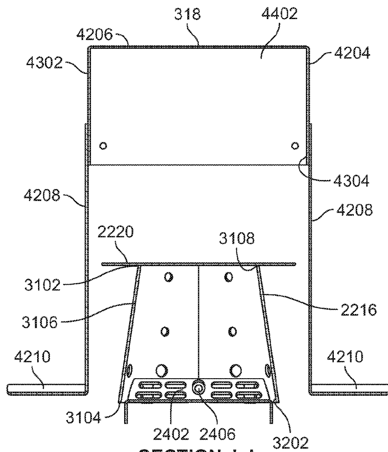
SECTION J-J
