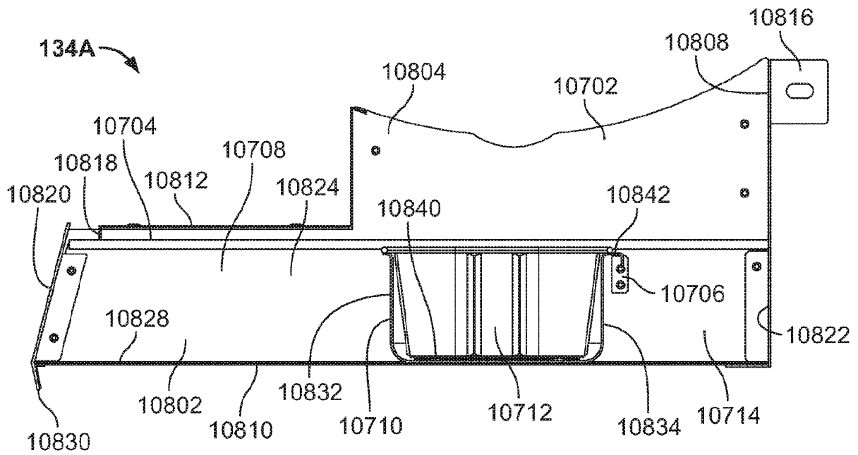
SECTION Y-Y
