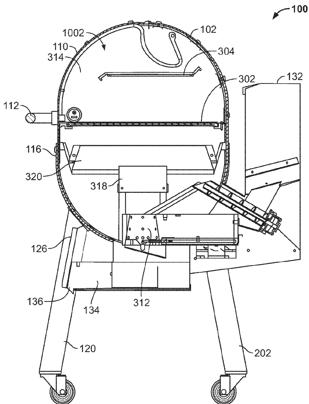
SECTION B-B
