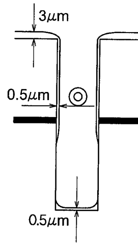
(b) Ion plating method
