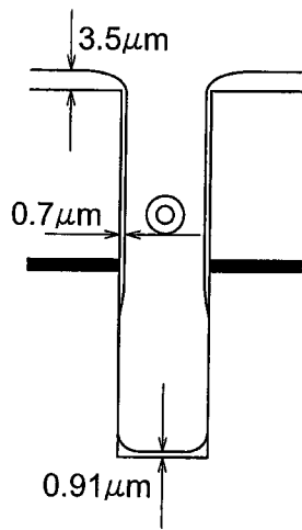
(c) Ion-beam sputtering method
