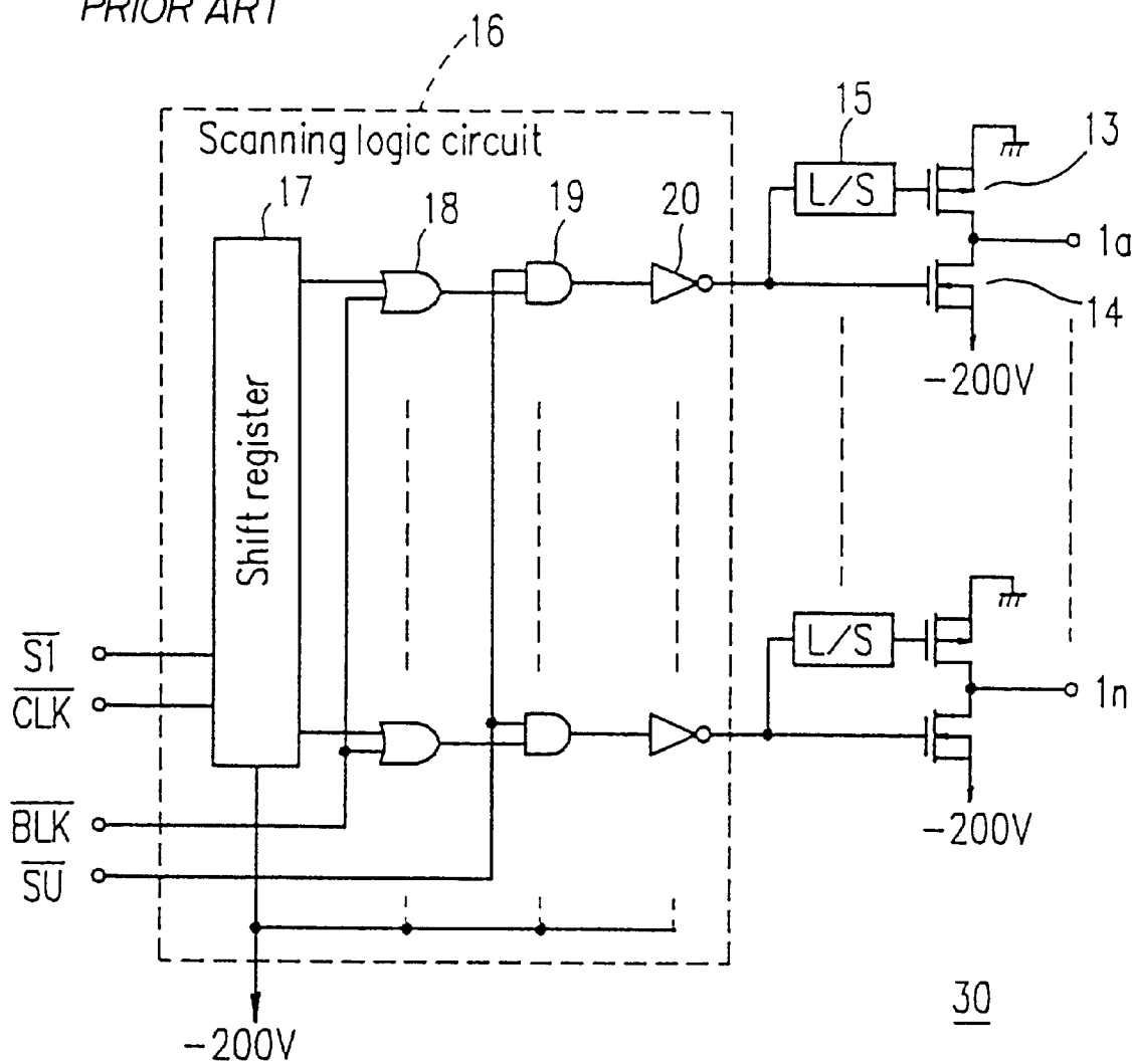
FIG. 6 PRIOR ART
