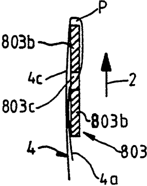
FIG. 2 (PRIOR ART)
