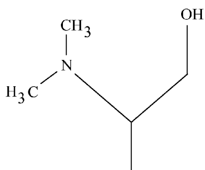
2-dimethylamino-1-propanol
