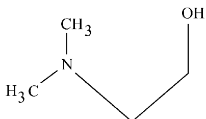
2-dimethylaminoethanol (DMEA)
