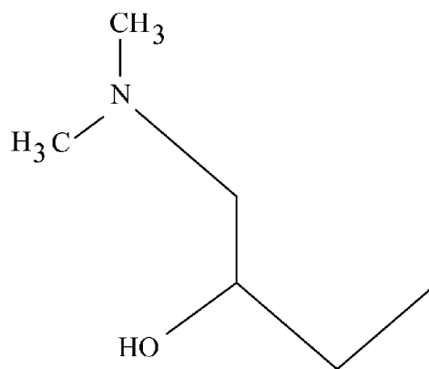
1-dimethylamino-2-butanol
