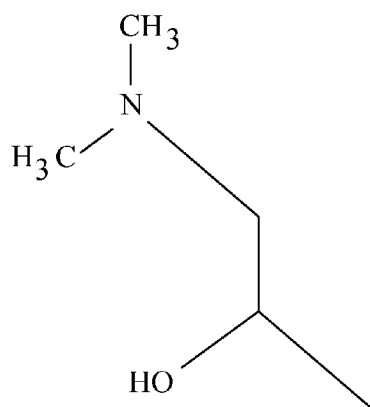
1-dimethylamino-2-propanol
