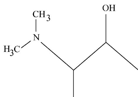
3-dimethylamino-2-butanol
