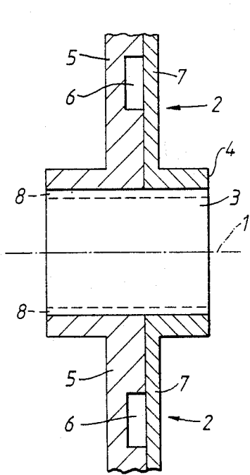
FIG. 1. PRIOR ART
