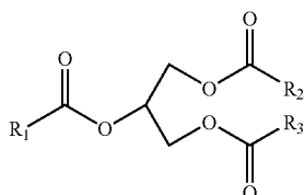
Structure of triglyceride
