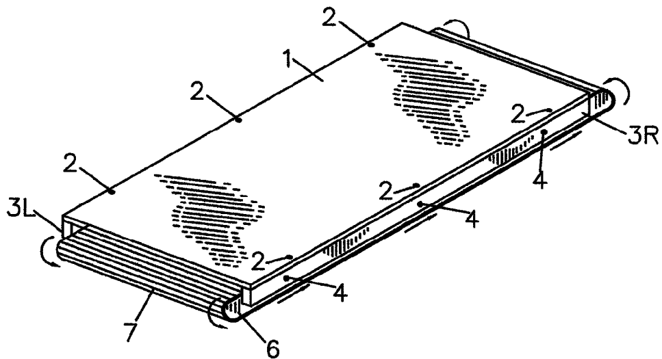
FIG. 2 SLIDE MECHANISM ASSEMBLED VIEW
