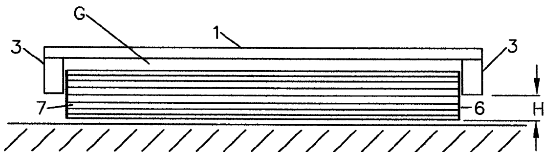
FIG. 3 SLIDE MECHANISM FRONT VIEW
