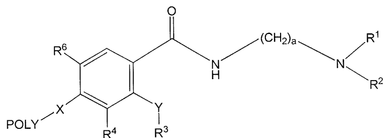
(Formula I-Cd)
