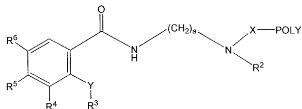
(Formula I-Ca)
