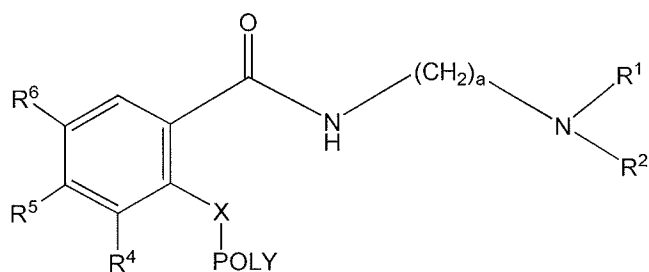
(Formula I-Cb)
