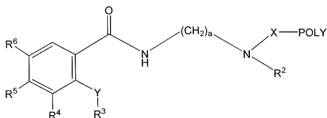
(Formula I-Ca)
