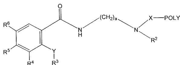
(Formula I-Ca)
