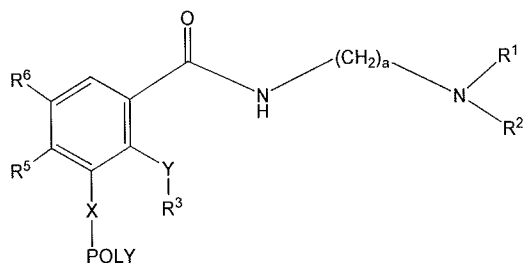
(Formula I-Cc)
