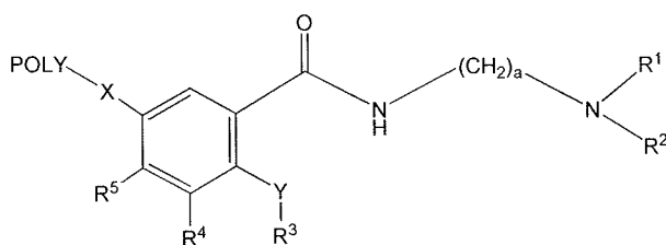
(Formula I-Ce)
