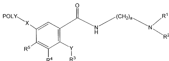
(Formula I-Ce)
