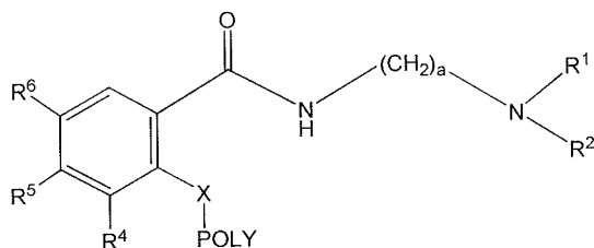
(Formula I-Cb)
