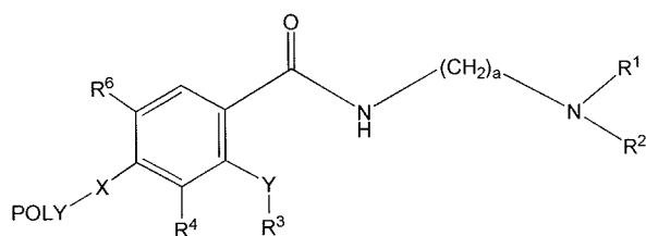
(Formula I-Cd)
