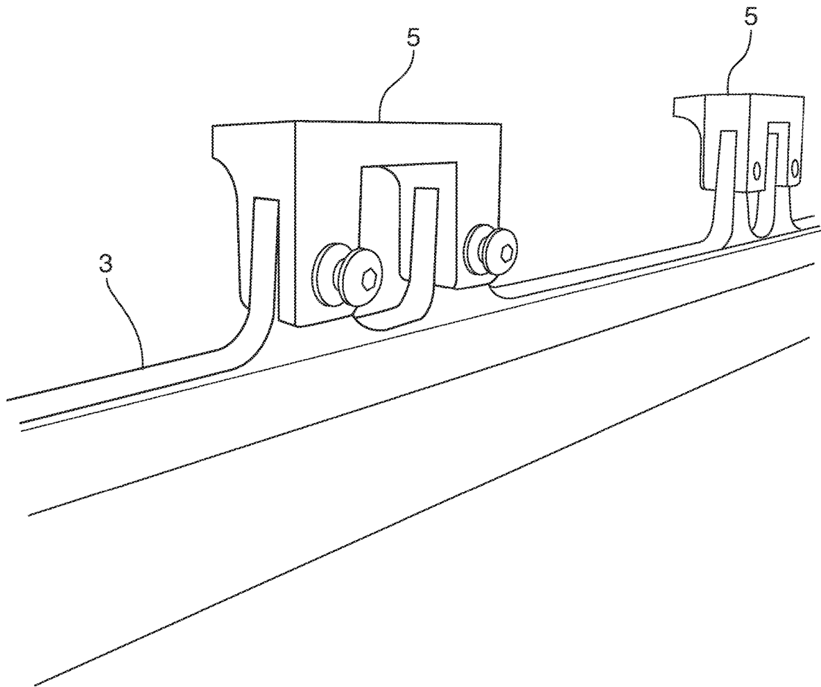
FIG. 2 Prior Art
