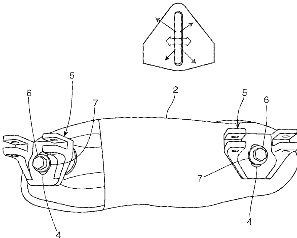
FIG. 3 Prior Art
