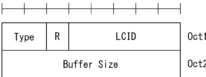
(b) MAC Control Elements
