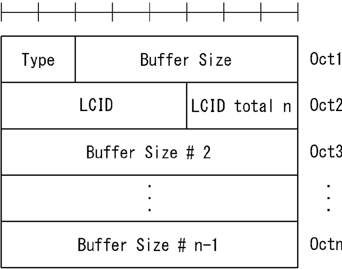
(b) MAC Control Elements
