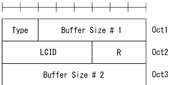
(b) MAC Control Elements - Type 2
