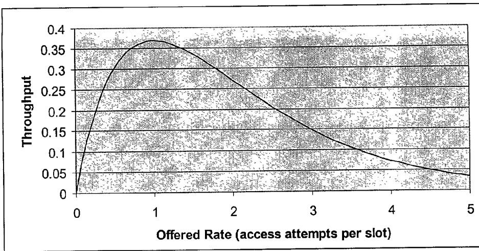
Figure 1. Throughput for a Slotted ALOHA Channel
