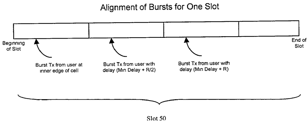
Figure 7 - Burst Alignment within Slotted ALOHA RACH
