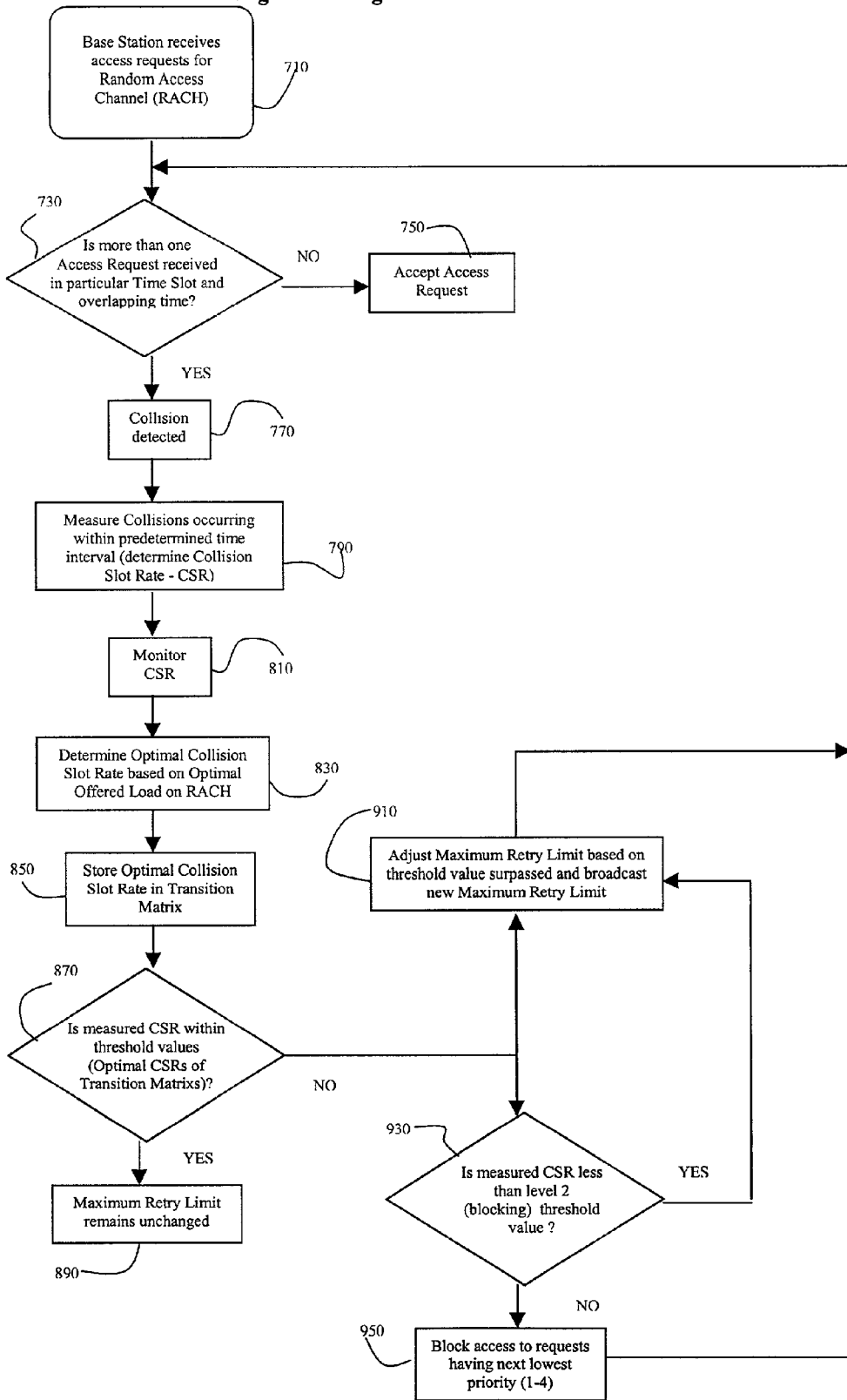
Figure 8 Congestion Control Process
