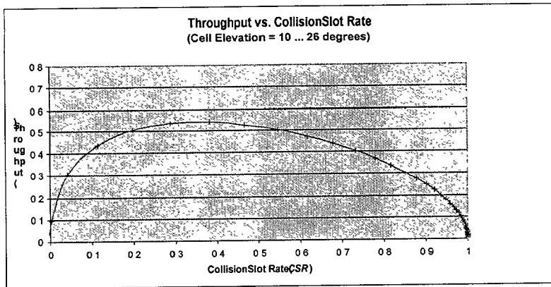
Figure 6 - CSR versus Throughput S
