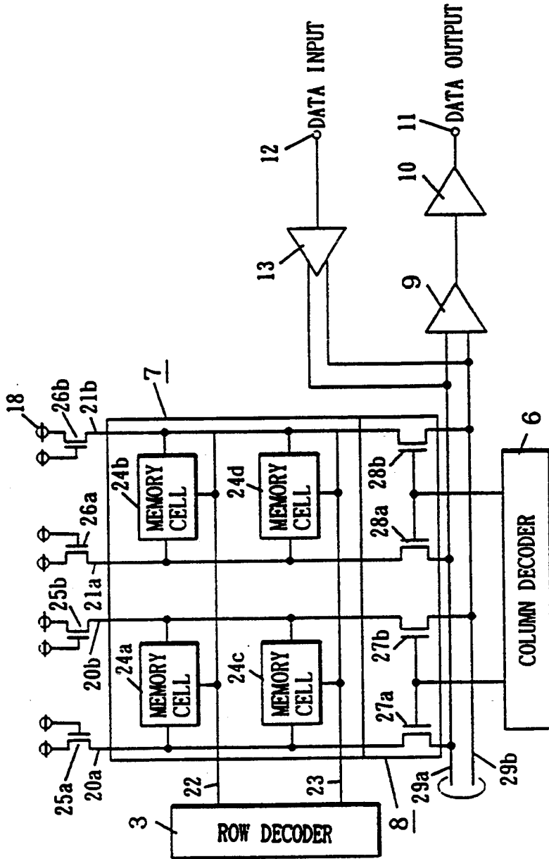
FIG. 46 PRIOR ART
