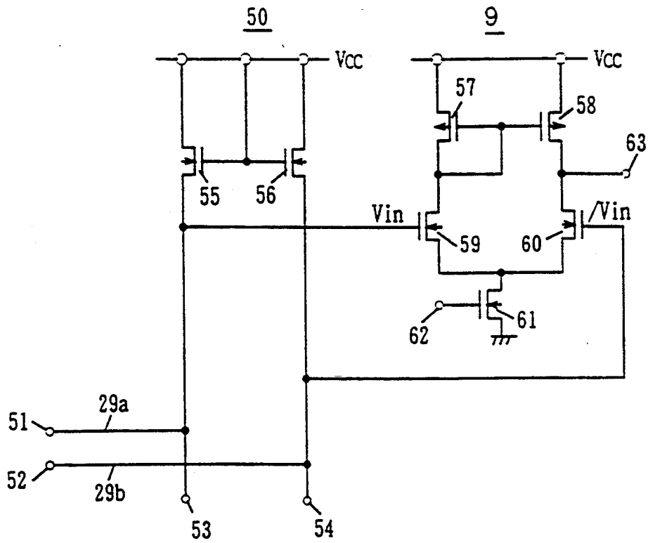
FIG. 49 PRIOR ART
