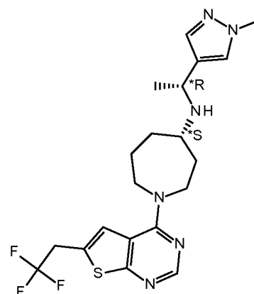
compound 54D
