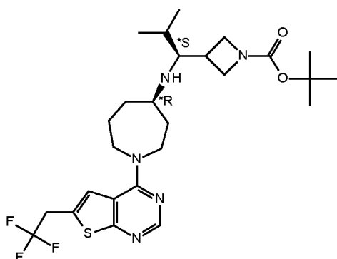
INTERMEDIATE 21A
