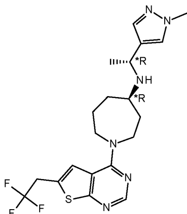
Compound 54A
