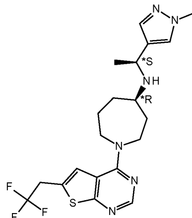
compound 54B
