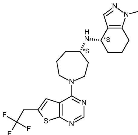
Compound 65D
