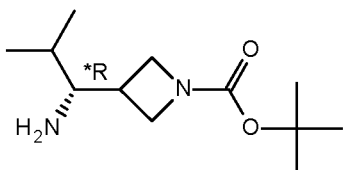
Intermediate 20A
