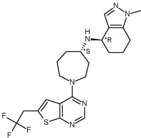
Compound 65C
