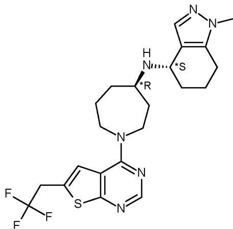
Compound 65B
