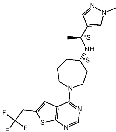
Compound 54C
