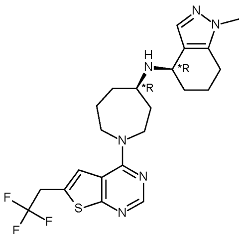
Compound 65A
