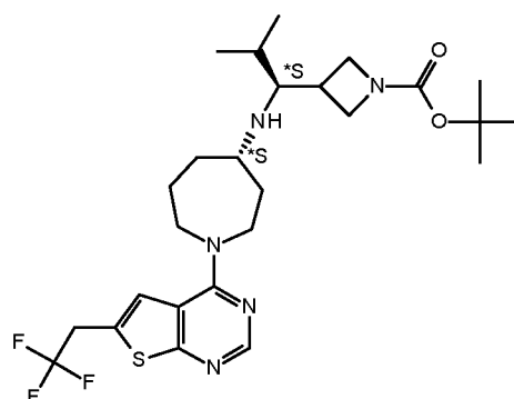
INTERMEDIATE 21B
