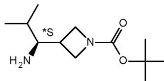
Intermediate 20B
