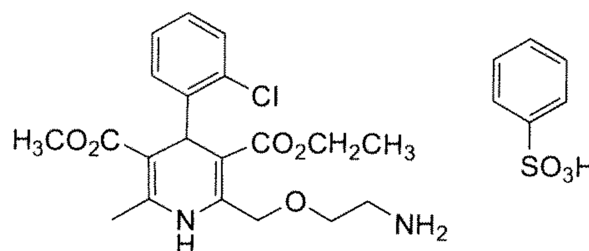
Amlodipine besylate
