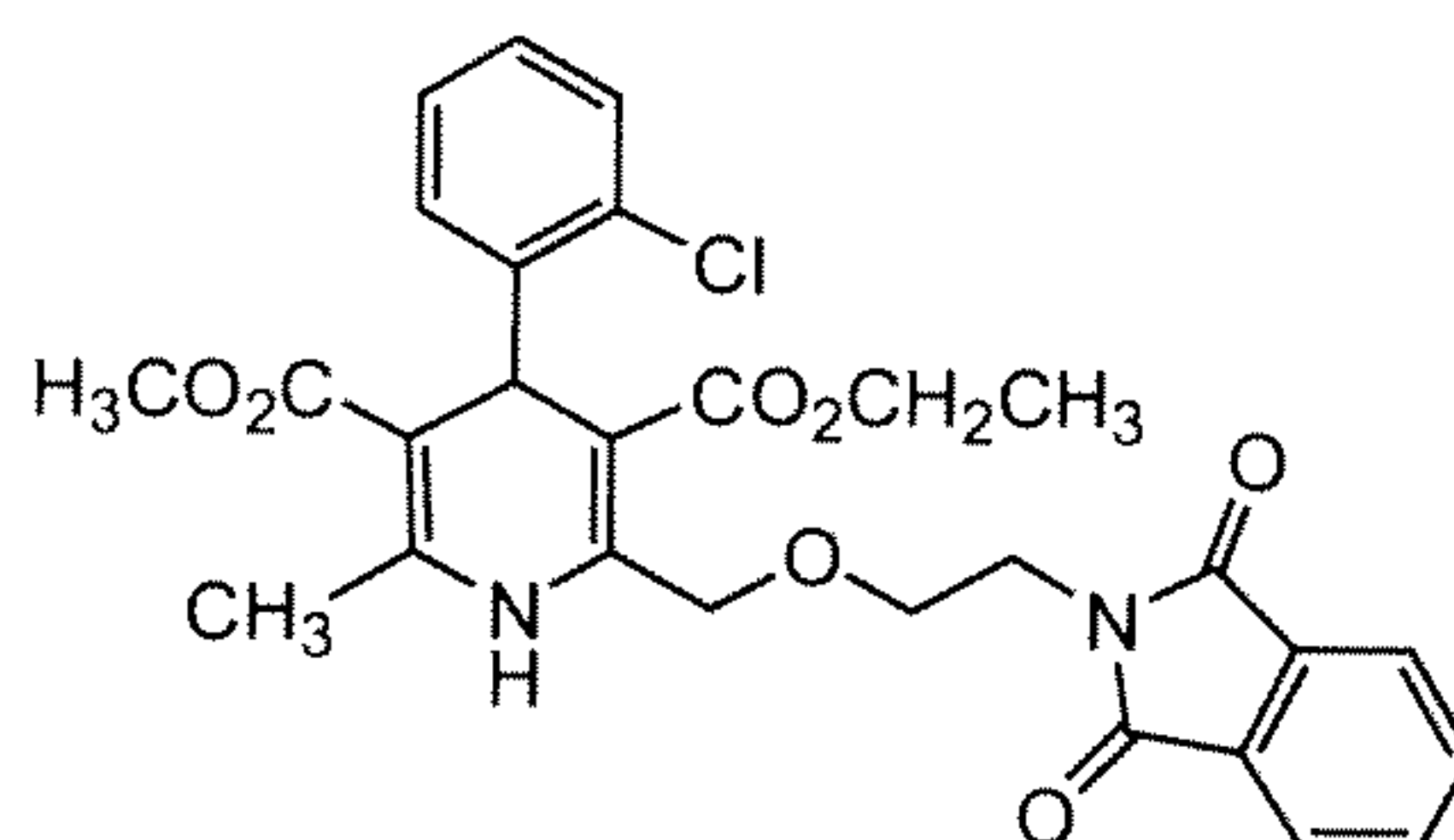
Phthaloyl amlodipine
