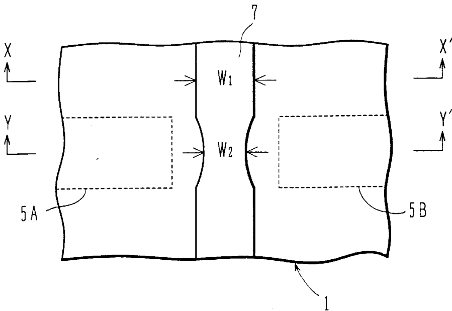
FIG.42 (PRIOR ART)
