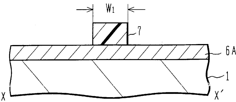
FIG.43 (PRIOR ART)
