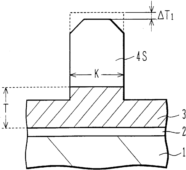
FIG.38 (PRIOR ART)
