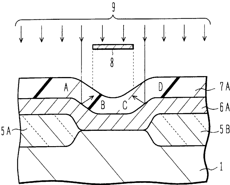
FIG.41 (PRIOR ART)
