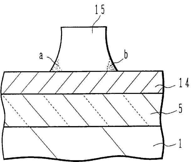
FIG.48 (PRIOR ART)
