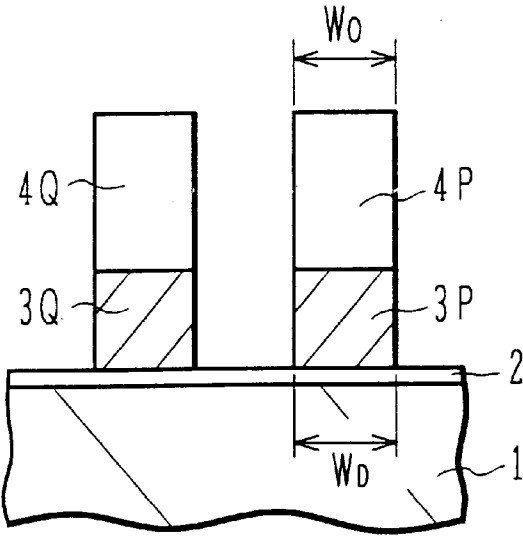
FIG.36 (PRIOR ART)
