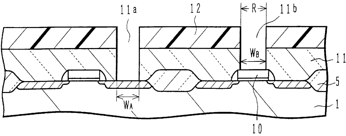
FIG.45 (PRIOR ART)
