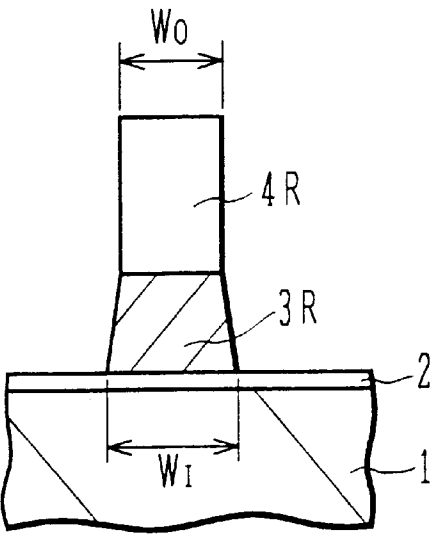
FIG.37 (PRIOR ART)
