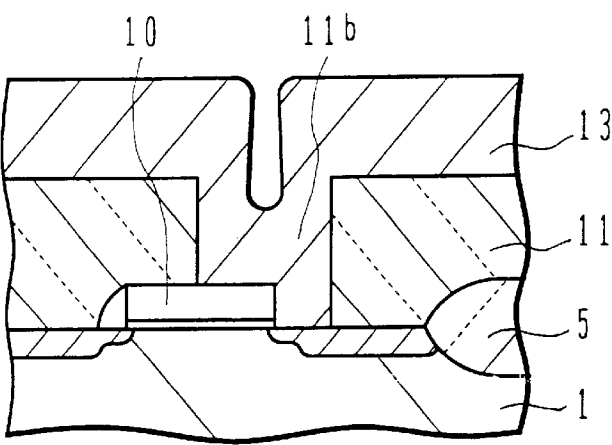
FIG.46 (PRIOR ART)
