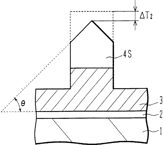
FIG.39 (PRIOR ART)
