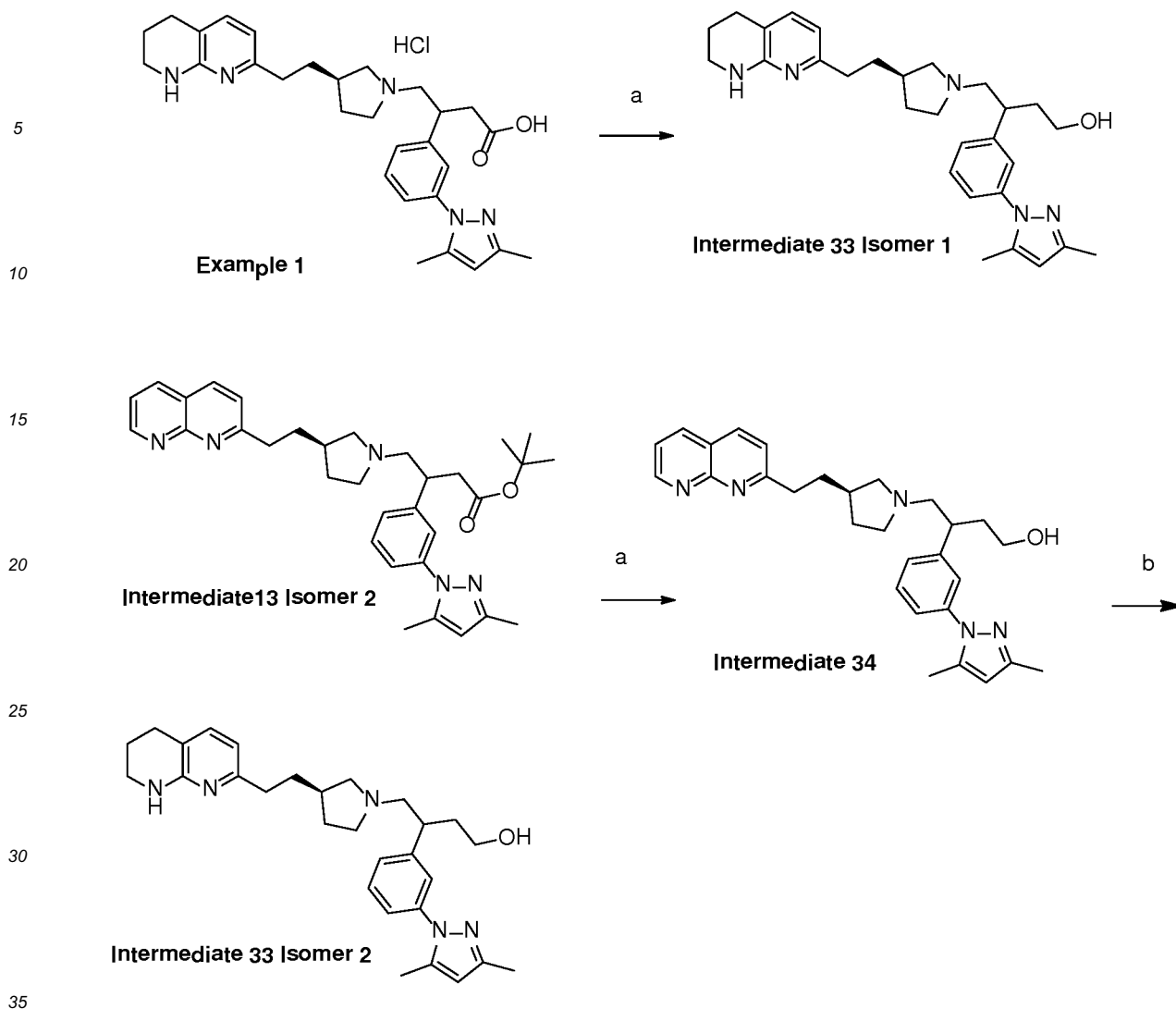
Scheme 3. Reagents and Conditions: (a) \text{LiAlH}_4 , THF; (b) \text{H}_2 , 5% Rh/C, EtOH
