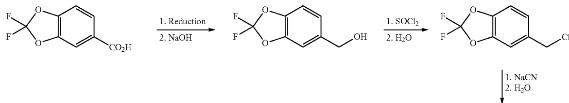
Scheme 1. Synthesis of the acid chloride moiety.
