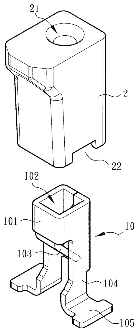
Fig. 1 PRIOR ART
