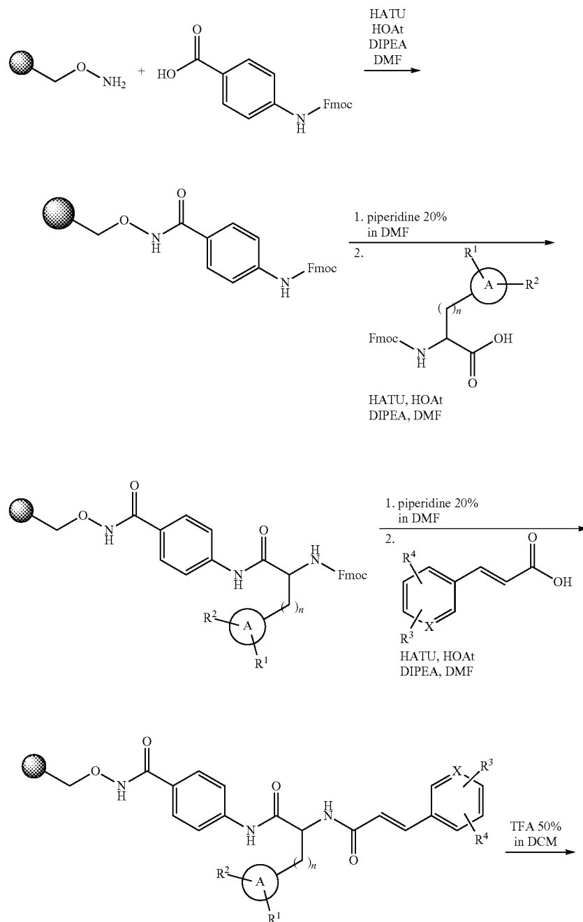
Scheme 1
