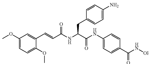
Compound 19D
