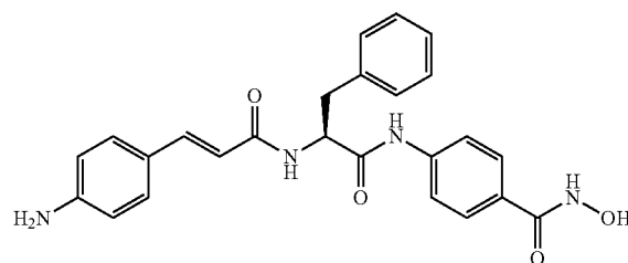
Compound 18D
