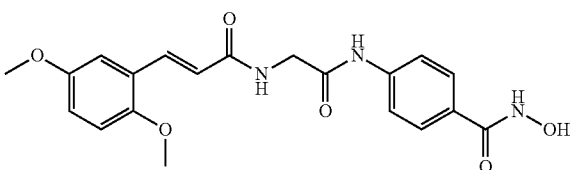
Compound 13D
