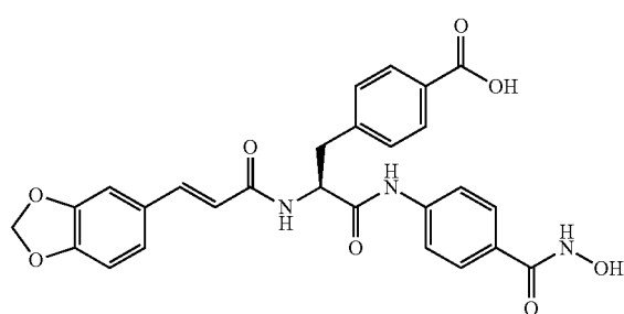
Compound 37D
