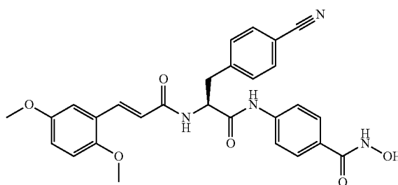
Compound 20D
