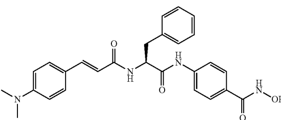
Compound 40D
