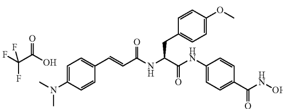
Compound 40D
