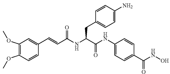
Compound 35D
