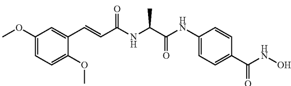
Compound 14D
