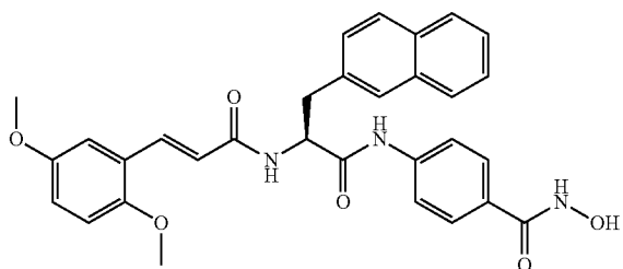
Compound 12D
