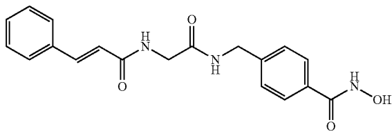
Compound 43D
