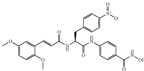
Compound 17D
