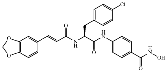
Compound 34D
