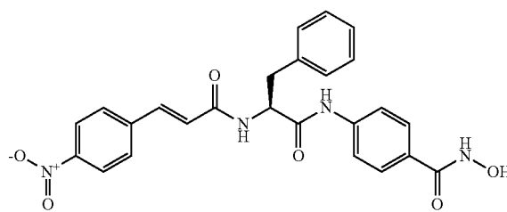
Compound 20D
