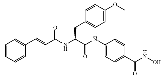
Compound 39D
