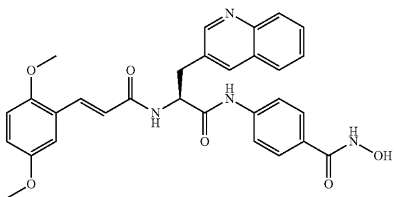
Compound 15D
