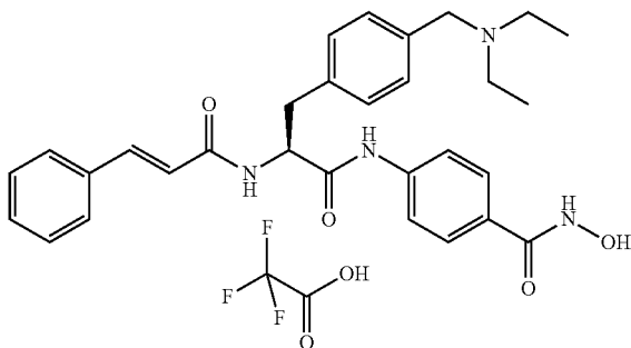
Compound 46D
