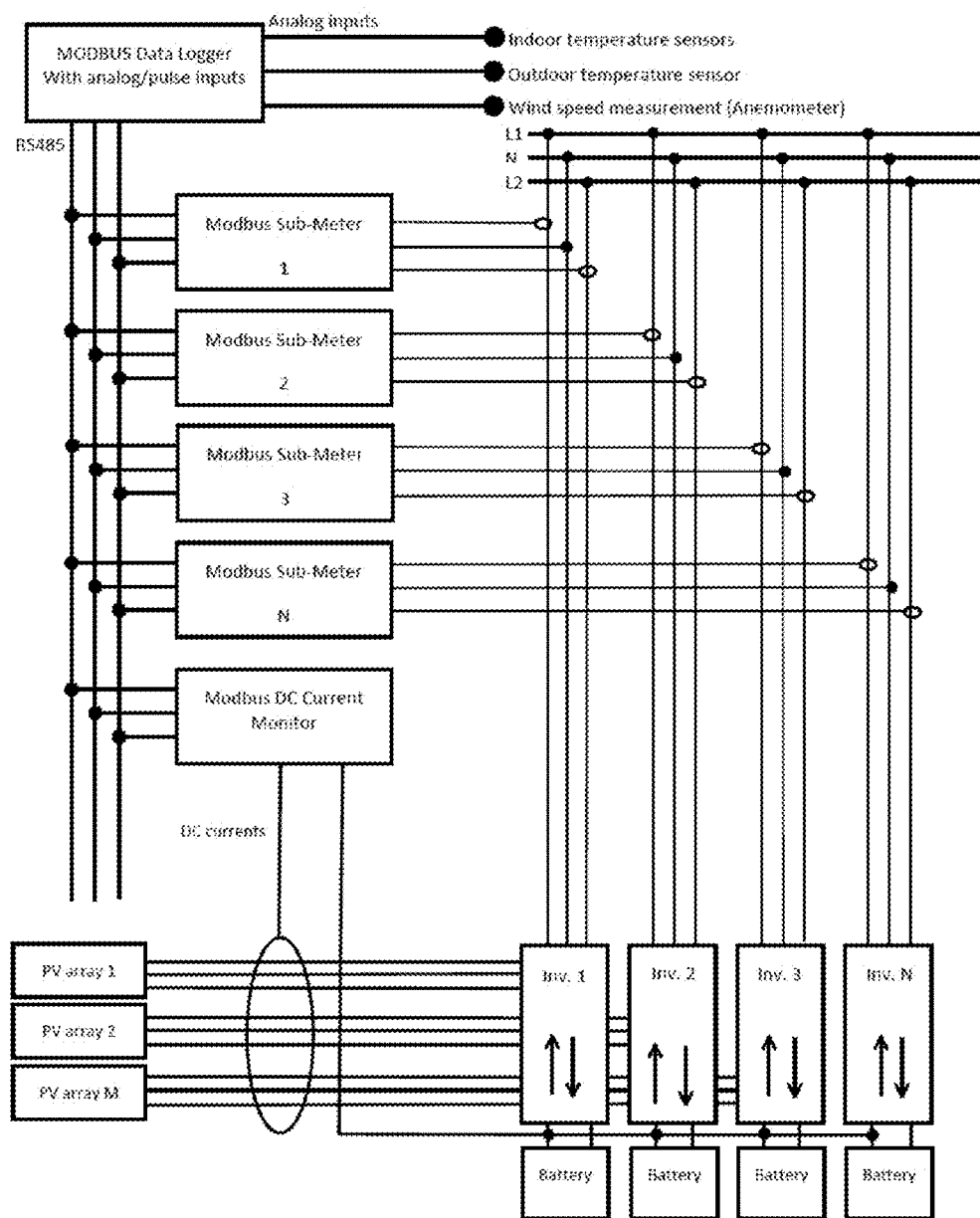
Figure 5 Outline of the local data logging system
