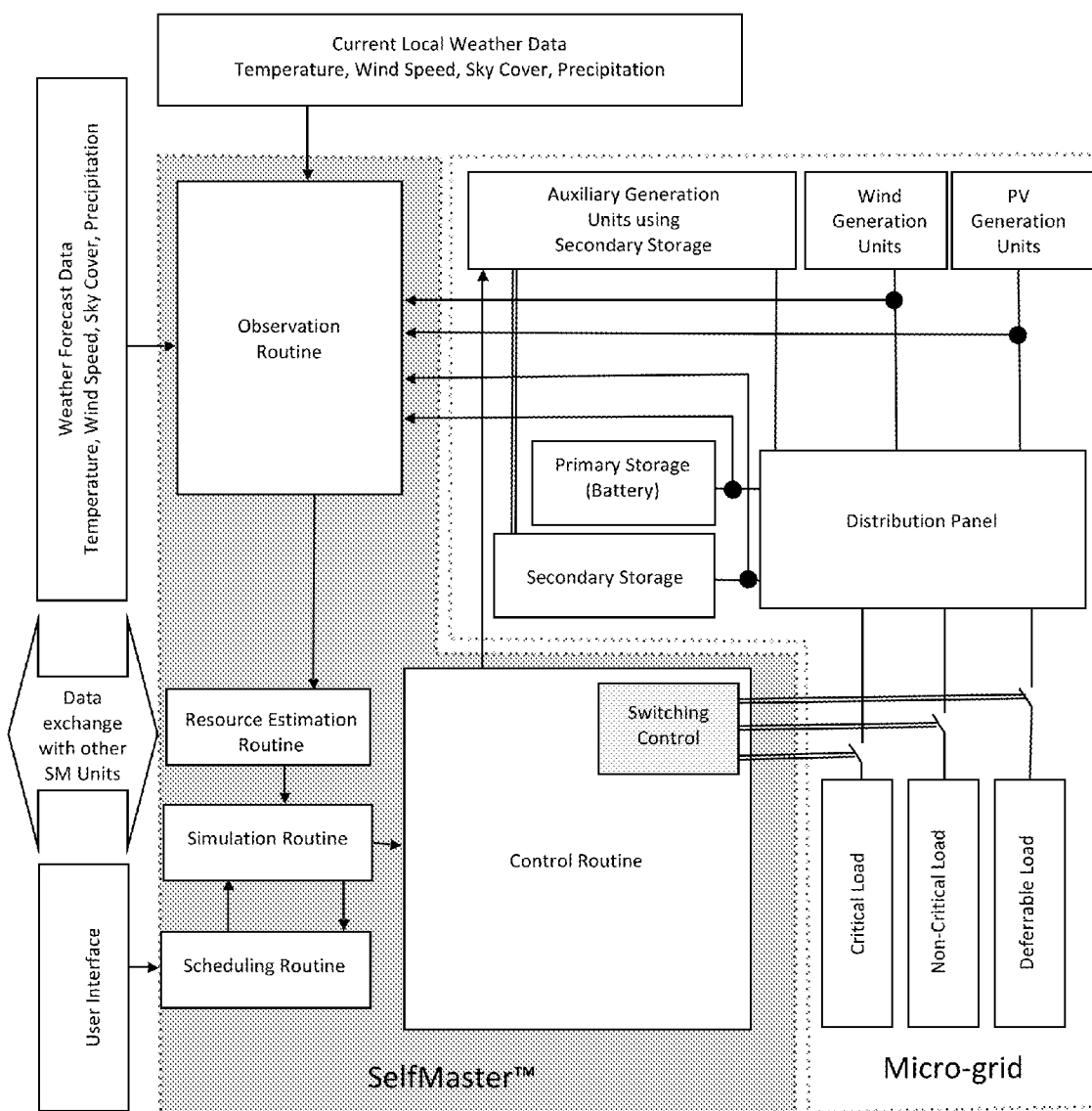
Figure 2 Interaction of SelfMaster™ with a micro-grid
