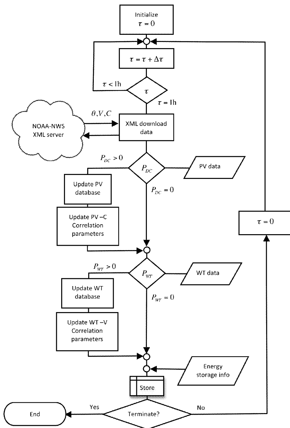
Figure 4 Flowchart of Observation Routine Operation
