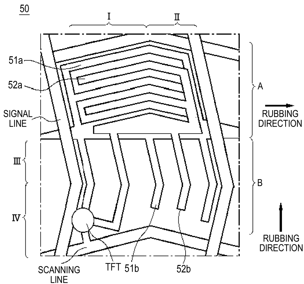
FIG. 10 PRIOR ART
