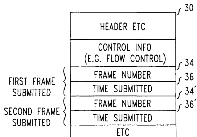
CONTROL FRAME (MAC-C TO MAC-D)
