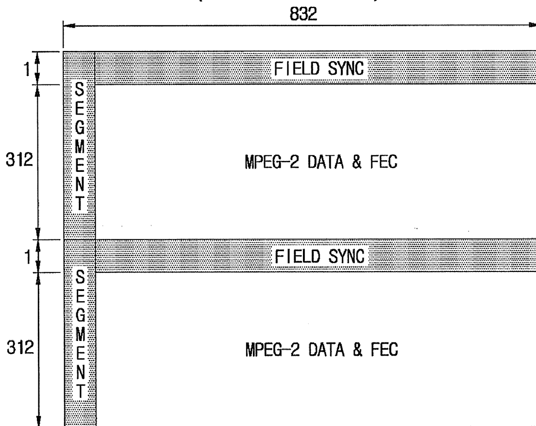
FIG. 2 (RELATED ART)
